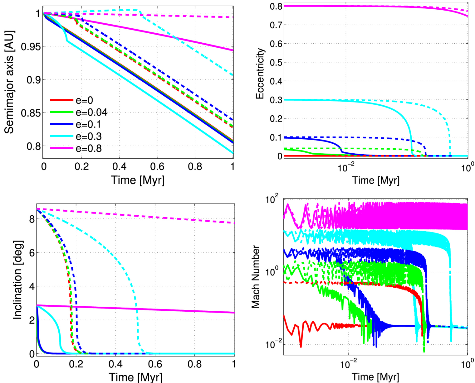
Figure 3. from APPLICATION OF GAS DYNAMICAL FRICTION FOR PLANETESIMALS. I. EVOLUTION OF SINGLE PLANETESIMALS null 2015 APJ 811 54 doi:10.1088/0004-637X/811/1/54 https://dx.doi.org/10.1088/0004-637X/811/1/54 © 2015. The American Astronomical Society. All rights reserved.
