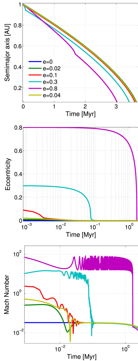
Figure 2. from APPLICATION OF GAS DYNAMICAL FRICTION FOR PLANETESIMALS. I. EVOLUTION OF SINGLE PLANETESIMALS null 2015 APJ 811 54 doi:10.1088/0004-637X/811/1/54 https://dx.doi.org/10.1088/0004-637X/811/1/54 © 2015. The American Astronomical Society. All rights reserved.
