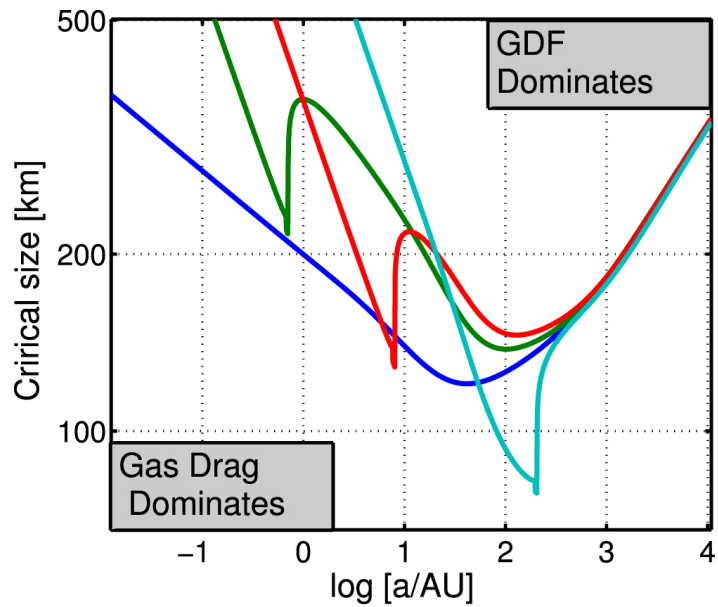
Figure 1. from APPLICATION OF GAS DYNAMICAL FRICTION FOR PLANETESIMALS. I. EVOLUTION OF SINGLE PLANETESIMALS null 2015 APJ 811 54 doi:10.1088/0004-637X/811/1/54 https://dx.doi.org/10.1088/0004-637X/811/1/54 © 2015. The American Astronomical Society. All rights reserved.
