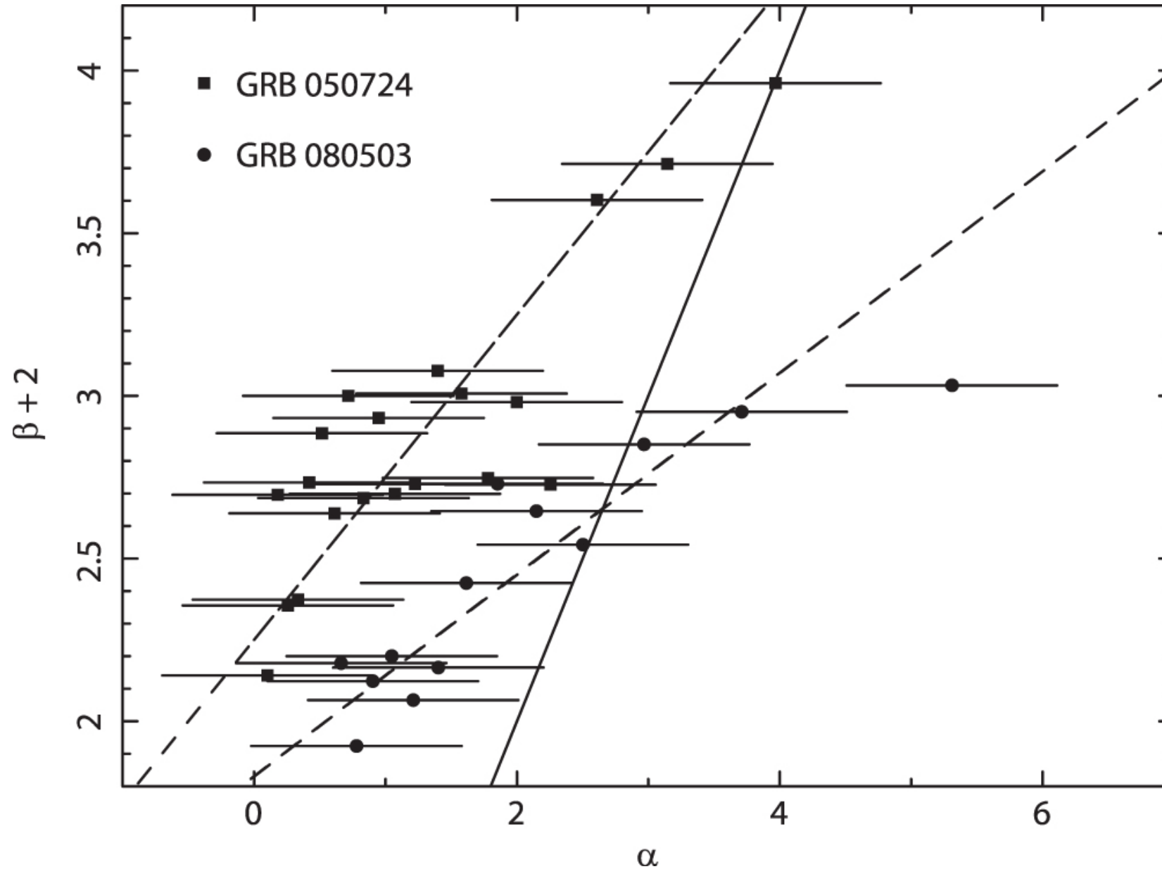
Figure 6. from X-RAYING EXTENDED EMISSION AND RAPID DECAY OF SHORT GAMMA-RAY BURSTS null 2015 APJ 811 4 doi:10.1088/0004-637X/811/1/4 https://dx.doi.org/10.1088/0004-637X/811/1/4 © 2015. The American Astronomical Society. All rights reserved.
