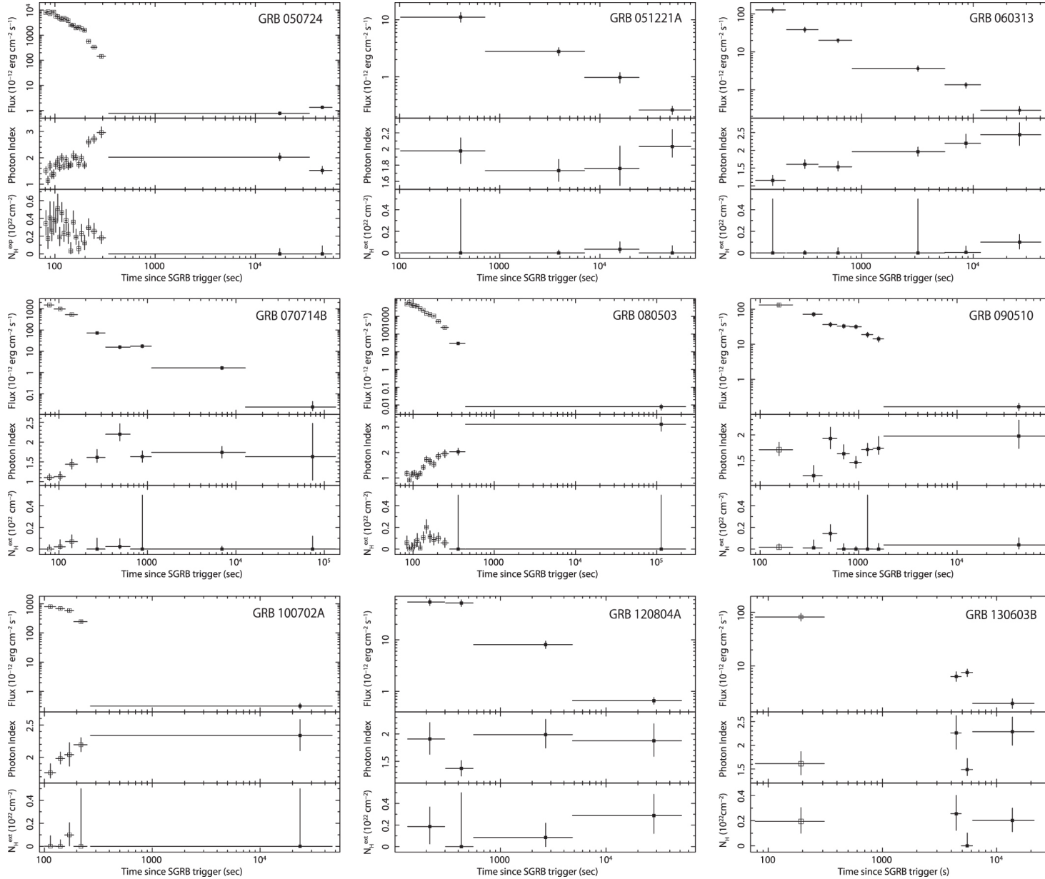
Figure 4. from X-RAYING EXTENDED EMISSION AND RAPID DECAY OF SHORT GAMMA-RAY BURSTS null 2015 APJ 811 4 doi:10.1088/0004-637X/811/1/4 https://dx.doi.org/10.1088/0004-637X/811/1/4 © 2015. The American Astronomical Society. All rights reserved.
