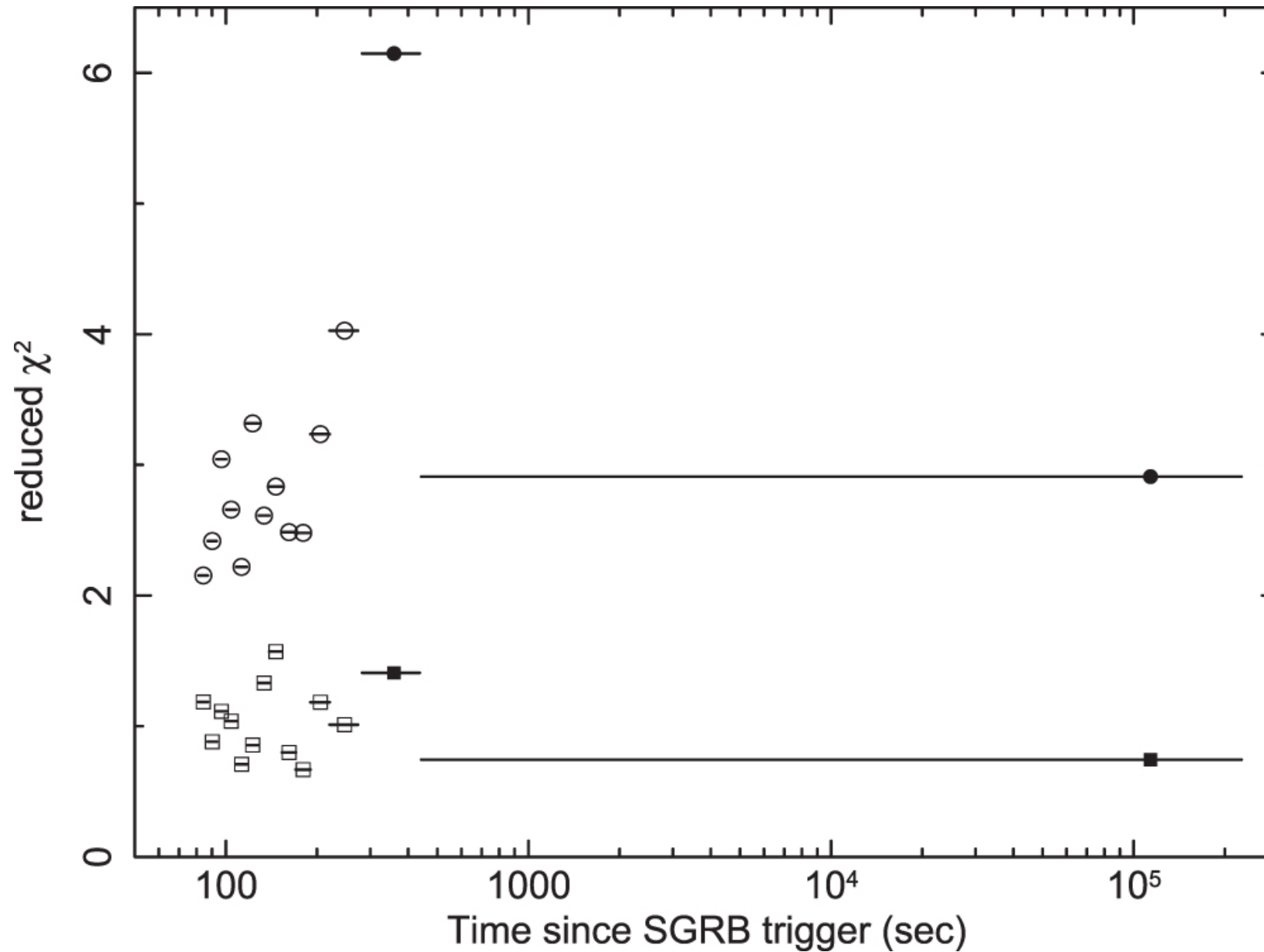
Figure 3. from X-RAYING EXTENDED EMISSION AND RAPID DECAY OF SHORT GAMMA-RAY BURSTS null 2015 APJ 811 4 doi:10.1088/0004-637X/811/1/4 https://dx.doi.org/10.1088/0004-637X/811/1/4 © 2015. The American Astronomical Society. All rights reserved.
