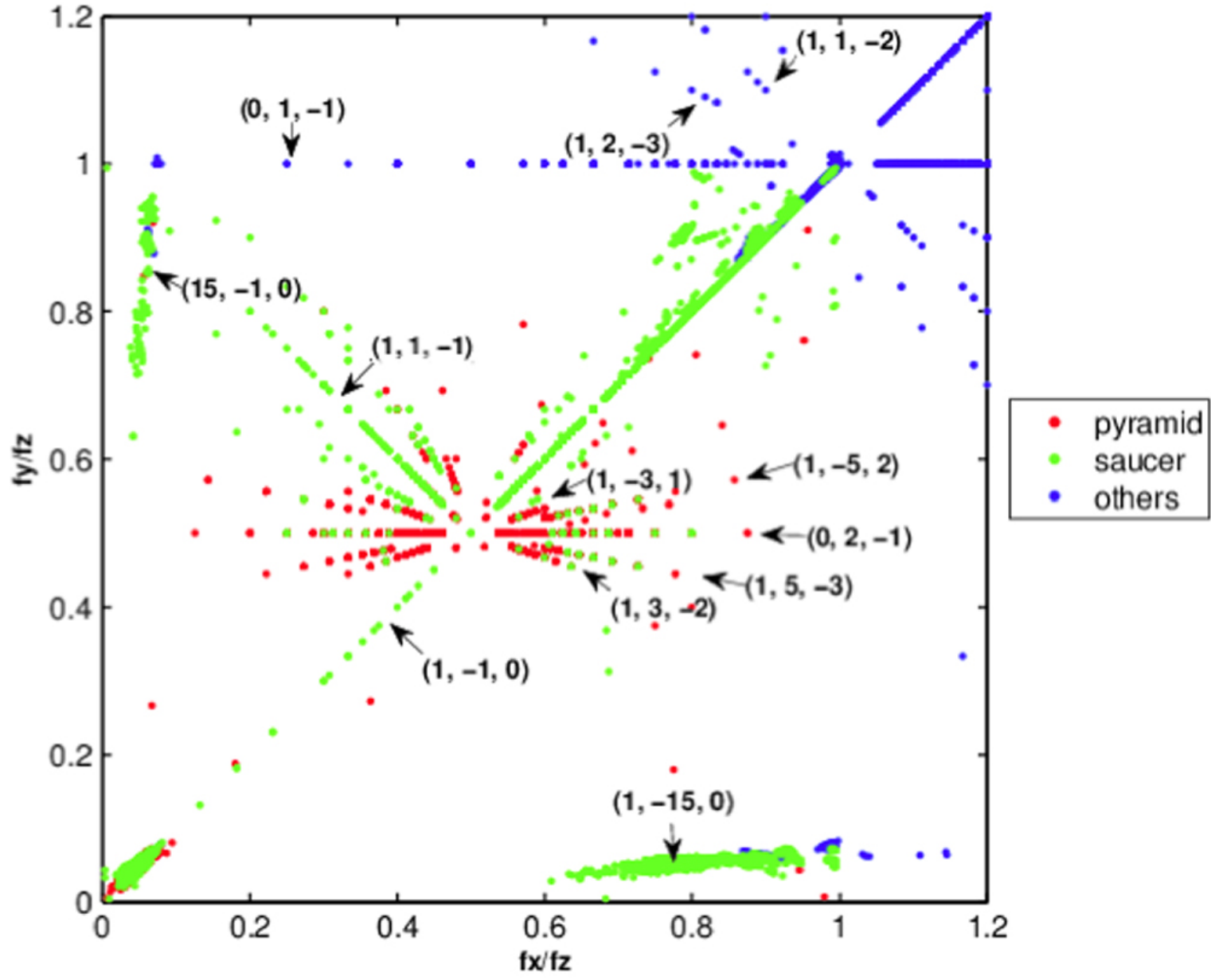
Figure 4. from CLASSIFICATION OF STELLAR ORBITS IN AXISYMMETRIC GALAXIES null 2015 APJ 811 25 doi:10.1088/0004-637X/811/1/25 https://dx.doi.org/10.1088/0004-637X/811/1/25 © 2015. The American Astronomical Society. All rights reserved.
