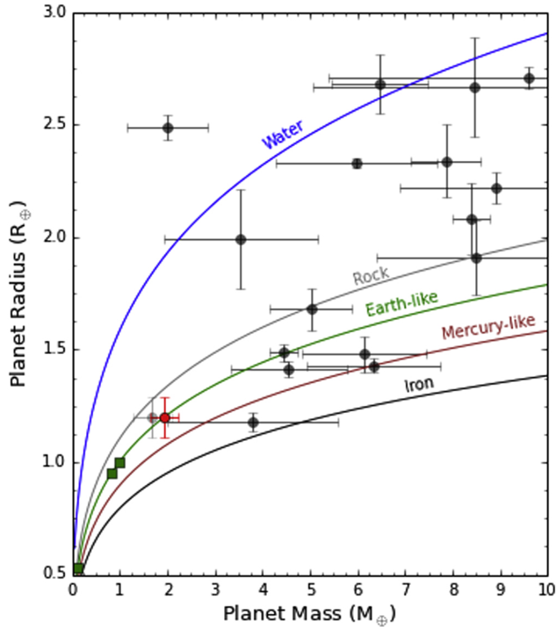
Figure 5. from DETERMINING THE MASS OF KEPLER-78b WITH NONPARAMETRIC GAUSSIAN PROCESS ESTIMATION null 2015 APJ 808 127 doi:10.1088/0004-637X/808/2/127 https://dx.doi.org/10.1088/0004-637X/808/2/127 © 2015. The American Astronomical Society. All rights reserved.
