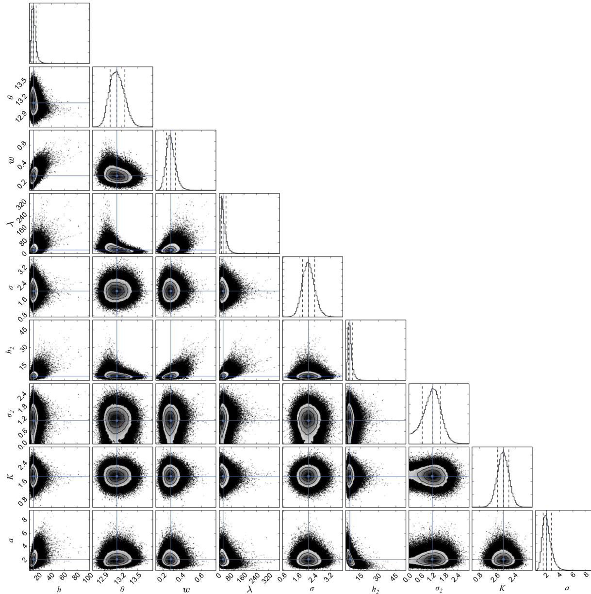
Figure 4. from DETERMINING THE MASS OF KEPLER-78b WITH NONPARAMETRIC GAUSSIAN PROCESS ESTIMATION null 2015 APJ 808 127 doi:10.1088/0004-637X/808/2/127 https://dx.doi.org/10.1088/0004-637X/808/2/127 © 2015. The American Astronomical Society. All rights reserved.
