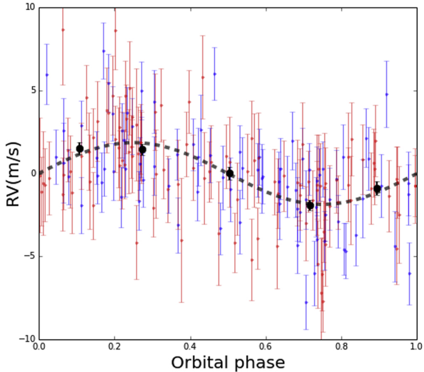
Figure 3. from DETERMINING THE MASS OF KEPLER-78b WITH NONPARAMETRIC GAUSSIAN PROCESS ESTIMATION null 2015 APJ 808 127 doi:10.1088/0004-637X/808/2/127 https://dx.doi.org/10.1088/0004-637X/808/2/127 © 2015. The American Astronomical Society. All rights reserved.
