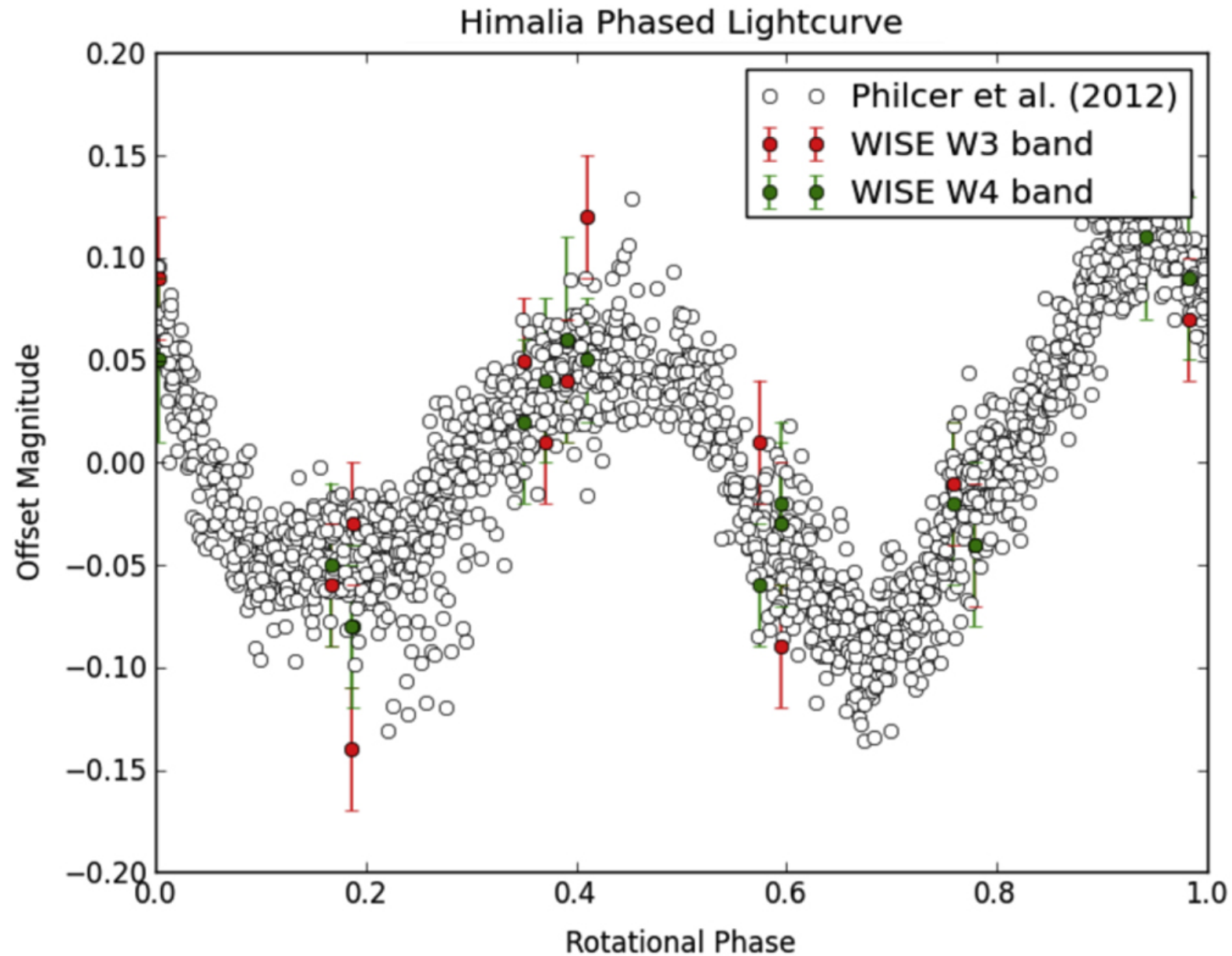
Figure 3. from NEOWISE: OBSERVATIONS OF THE IRREGULAR SATELLITES OF JUPITER AND SATURN null 2015 APJ 809 3 doi:10.1088/0004-637X/809/1/3 https://dx.doi.org/10.1088/0004-637X/809/1/3 © 2015. The American Astronomical Society. All rights reserved.
