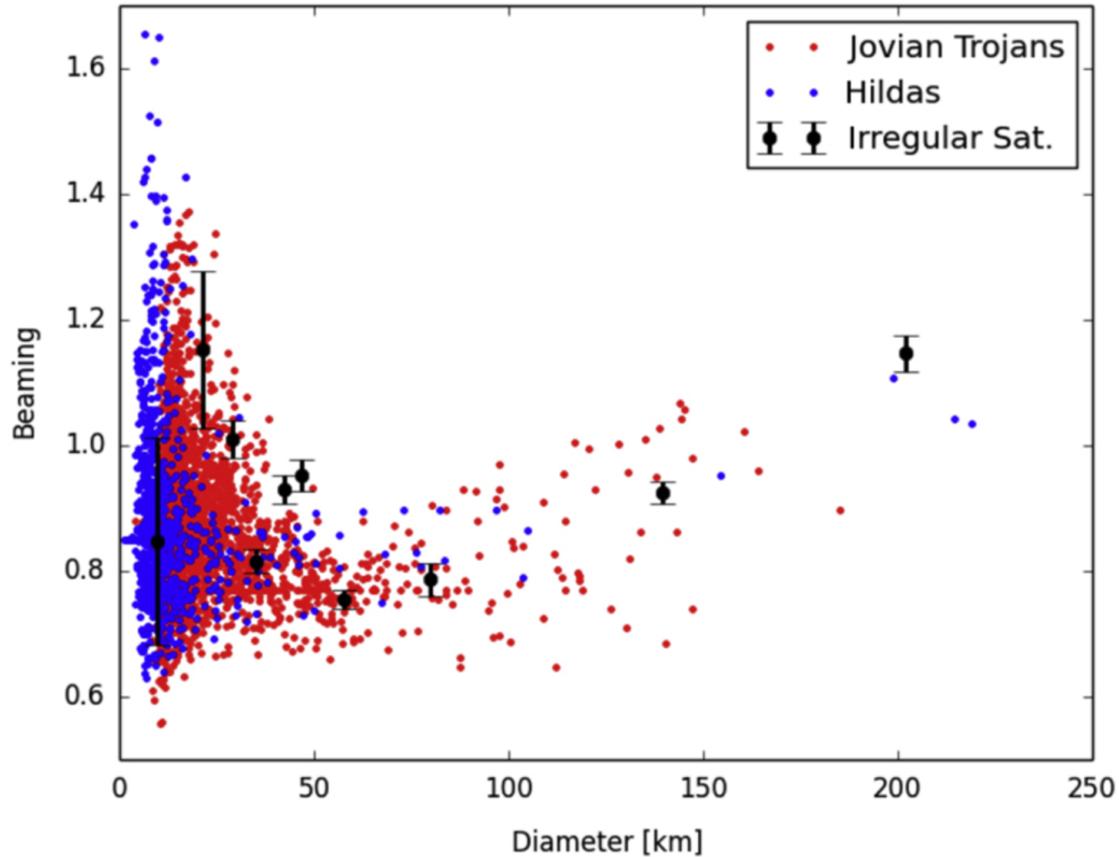
Figure 2. from NEOWISE: OBSERVATIONS OF THE IRREGULAR SATELLITES OF JUPITER AND SATURN null 2015 APJ 809 3 doi:10.1088/0004-637X/809/1/3 https://dx.doi.org/10.1088/0004-637X/809/1/3 © 2015. The American Astronomical Society. All rights reserved.
