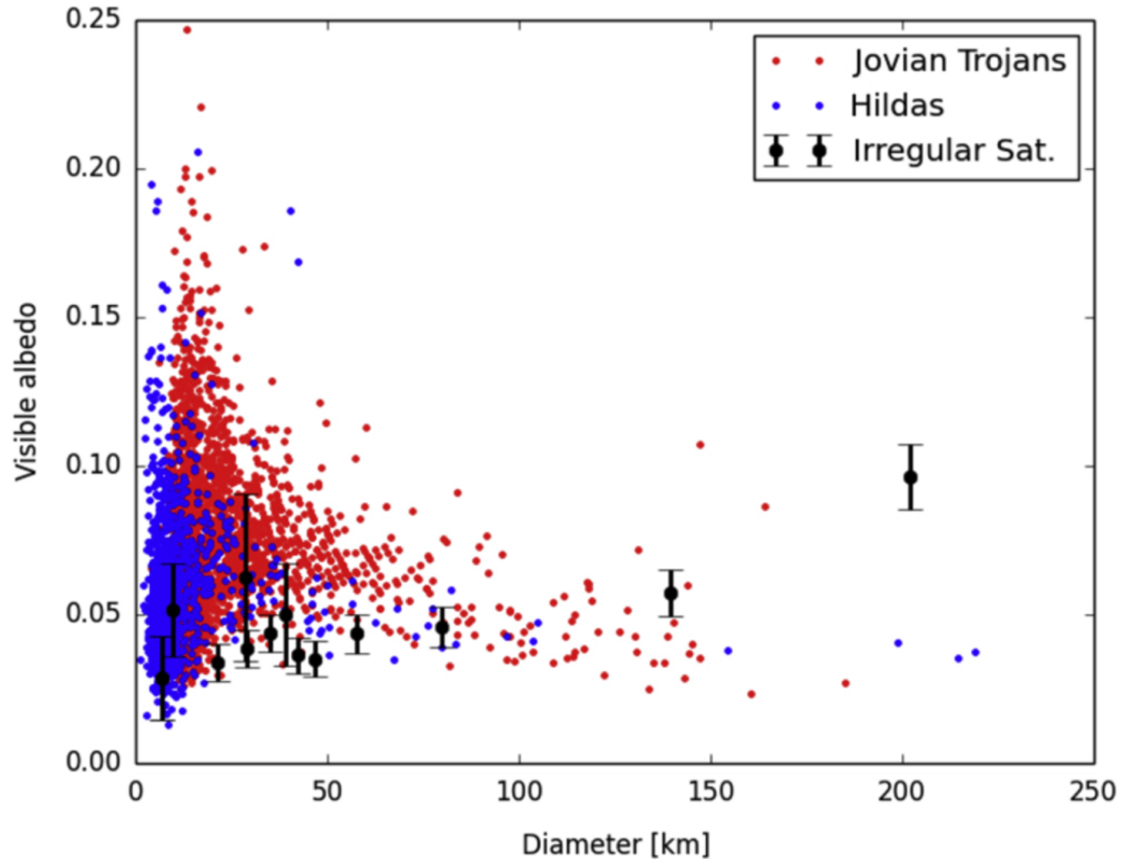
Figure 1. from NEOWISE: OBSERVATIONS OF THE IRREGULAR SATELLITES OF JUPITER AND SATURN null 2015 APJ 809 3 doi:10.1088/0004-637X/809/1/3 https://dx.doi.org/10.1088/0004-637X/809/1/3 © 2015. The American Astronomical Society. All rights reserved.
