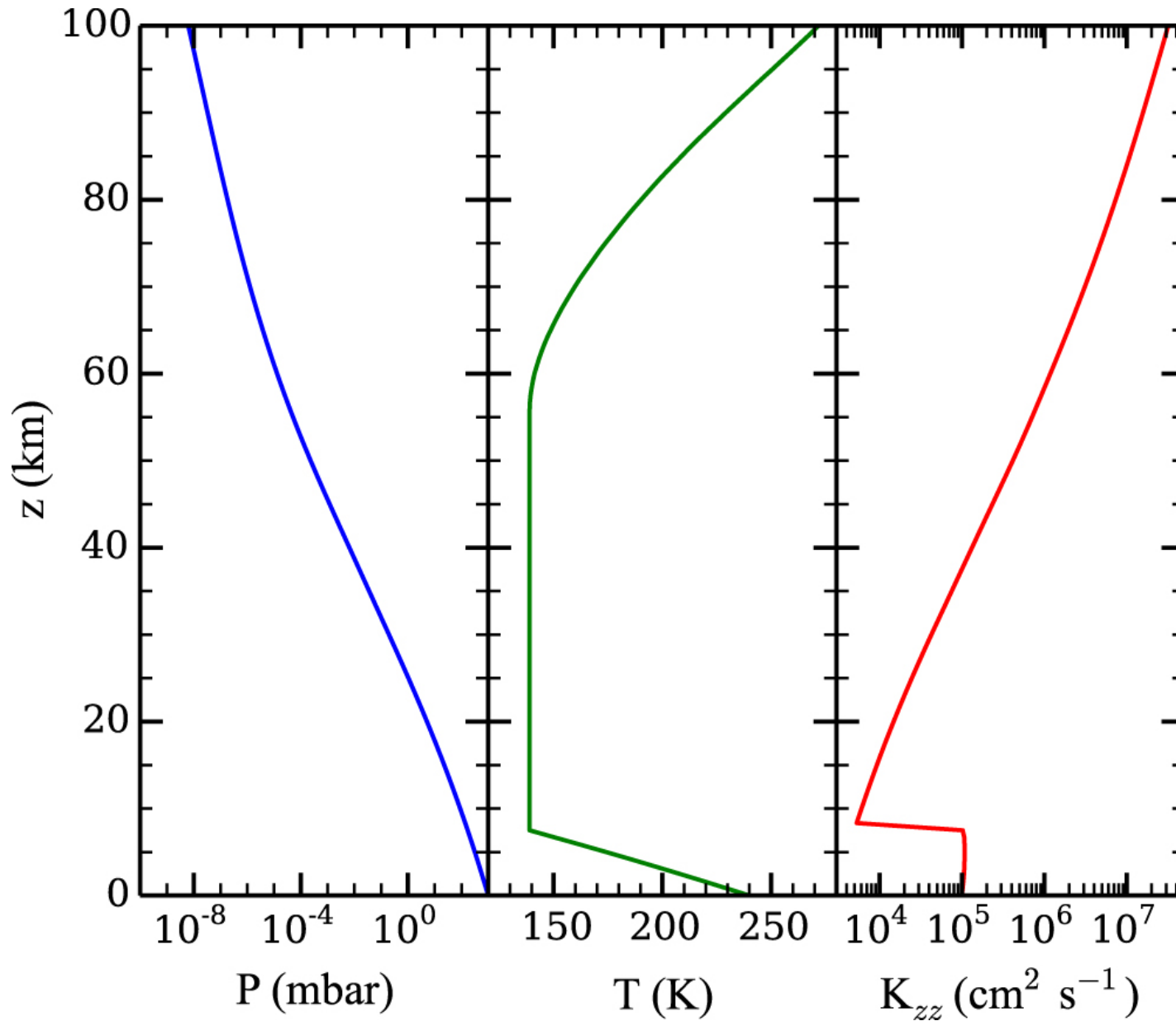
Figure 2. from STABILITY OF CO 2 ATMOSPHERES ON DESICCATED M DWARF EXOPLANETS null 2015 APJ 806 249 doi:10.1088/0004-637X/806/2/249 https://dx.doi.org/10.1088/0004-637X/806/2/249 © 2015. The American Astronomical Society. All rights reserved.
