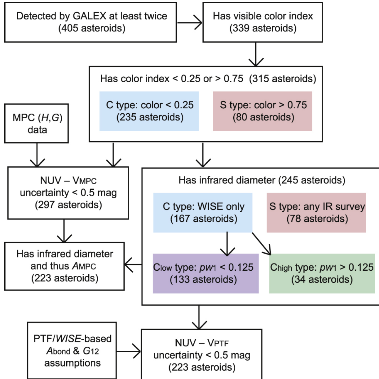
Figure 5. from ASTEROIDS IN GALEX: NEAR-ULTRAVIOLET PHOTOMETRY OF THE MAJOR TAXONOMIC GROUPS null 2015 APJ 809 92 doi:10.1088/0004-637X/809/1/92 https://dx.doi.org/10.1088/0004-637X/809/1/92 © 2015. The American Astronomical Society. All rights reserved.
