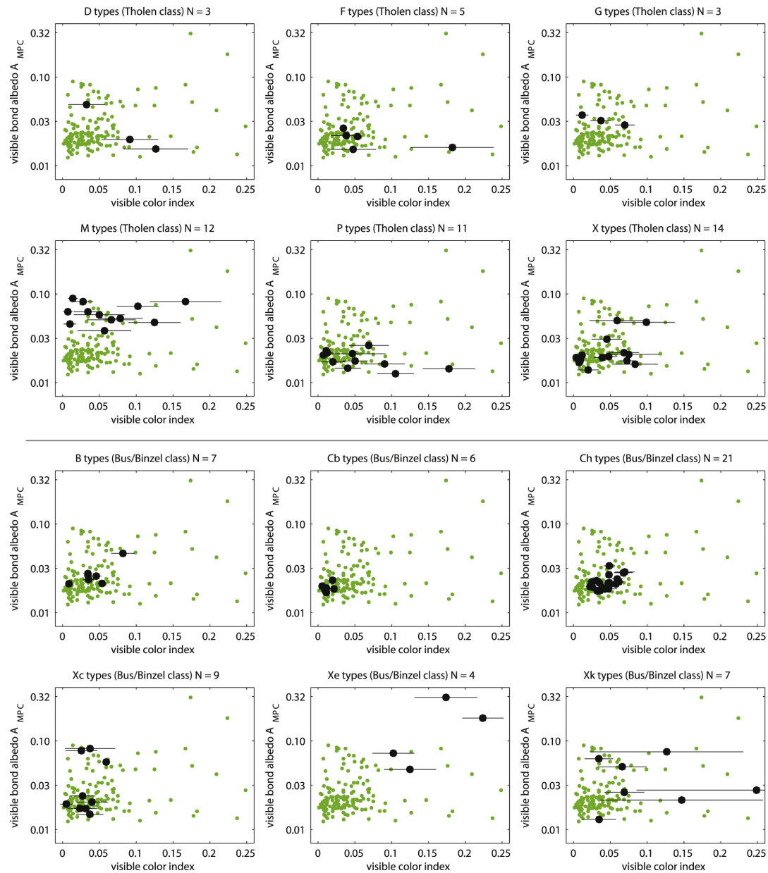
Figure 10. from ASTEROIDS IN GALEX: NEAR-ULTRAVIOLET PHOTOMETRY OF THE MAJOR TAXONOMIC GROUPS null 2015 APJ 809 92 doi:10.1088/0004-637X/809/1/92 https://dx.doi.org/10.1088/0004-637X/809/1/92
