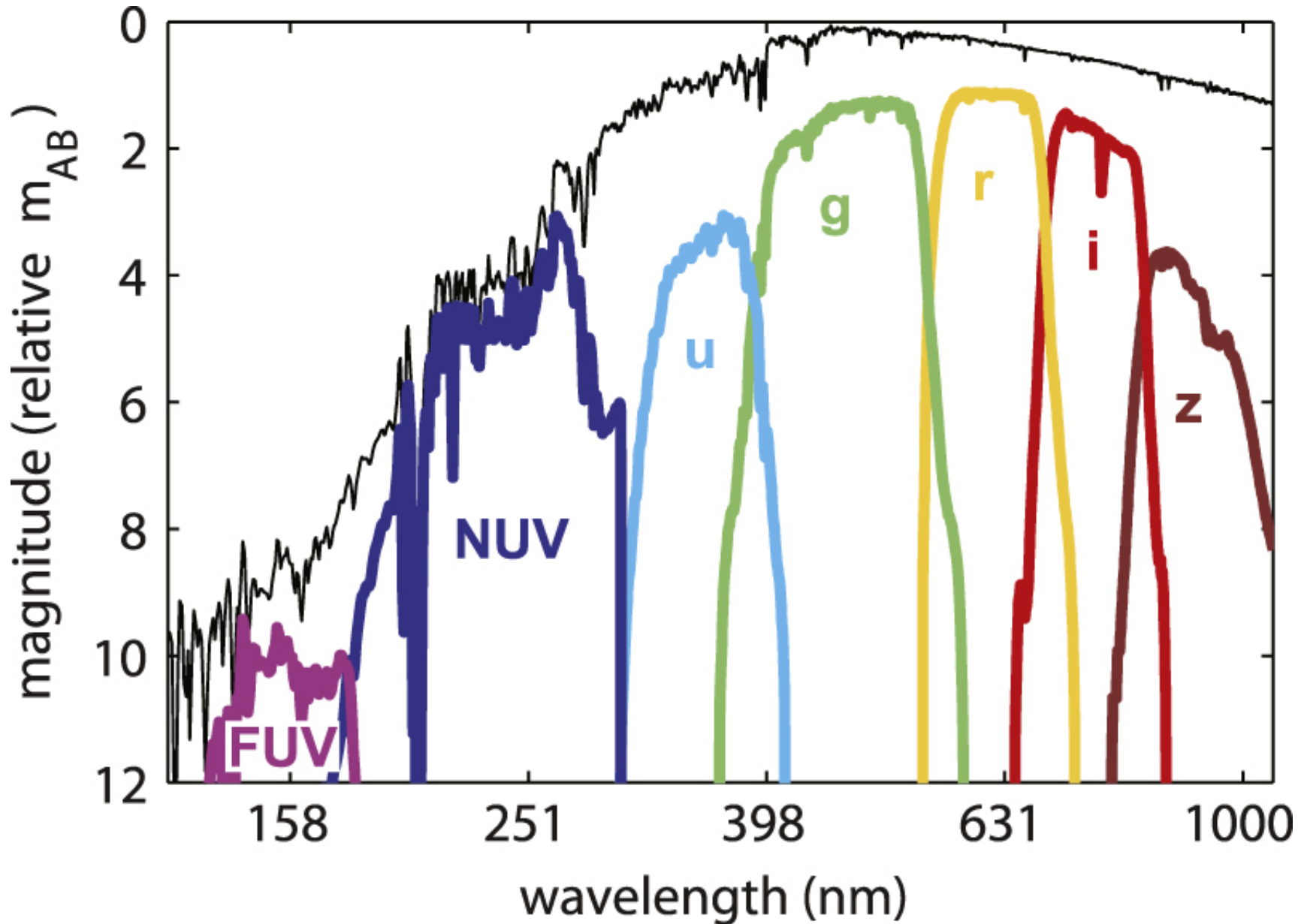
Figure 1. from ASTEROIDS IN GALEX: NEAR-ULTRAVIOLET PHOTOMETRY OF THE MAJOR TAXONOMIC GROUPS null 2015 APJ 809 92 doi:10.1088/0004-637X/809/1/92 https://dx.doi.org/10.1088/0004-637X/809/1/92 © 2015. The American Astronomical Society. All rights reserved.
