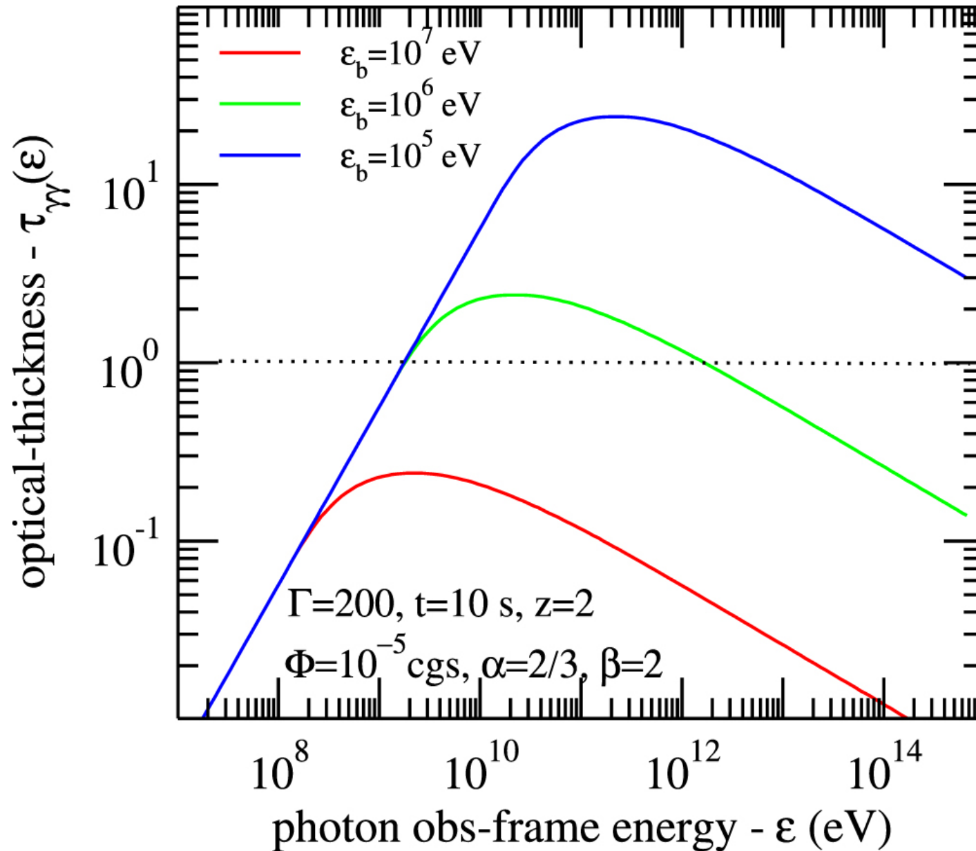
Figure 1. from OPTICAL FLASHES FROM INTERNAL PAIRS FORMED IN GAMMA-RAY BURST AFTERGLOWS null 2015 APJ 806 64 doi:10.1088/0004-637X/806/1/64 https://dx.doi.org/10.1088/0004-637X/806/1/64 © 2015. The American Astronomical Society. All rights reserved.
