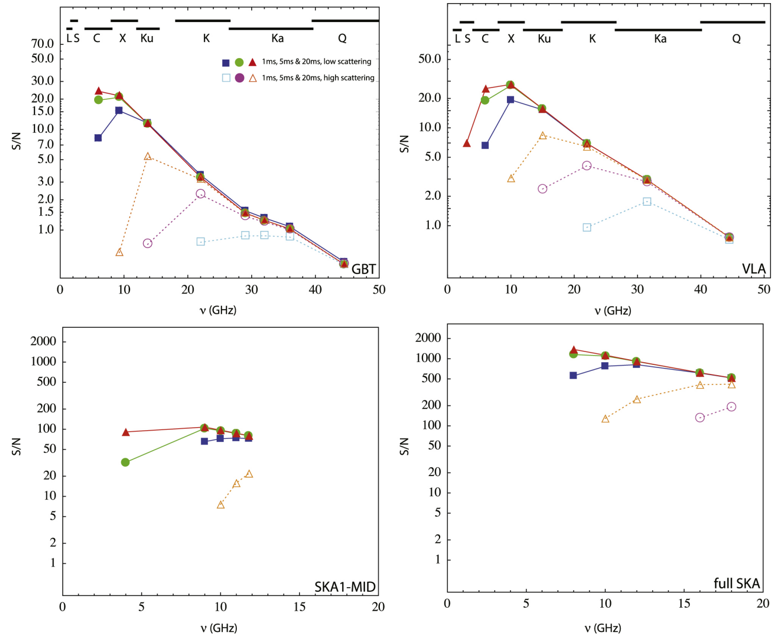
Figure 2. from ON DETECTING MILLISECOND PULSARS AT THE GALACTIC CENTER null 2015 APJ 805 172 doi:10.1088/0004-637X/805/2/172 https://dx.doi.org/10.1088/0004-637X/805/2/172 © 2015. The American Astronomical Society. All rights reserved.
