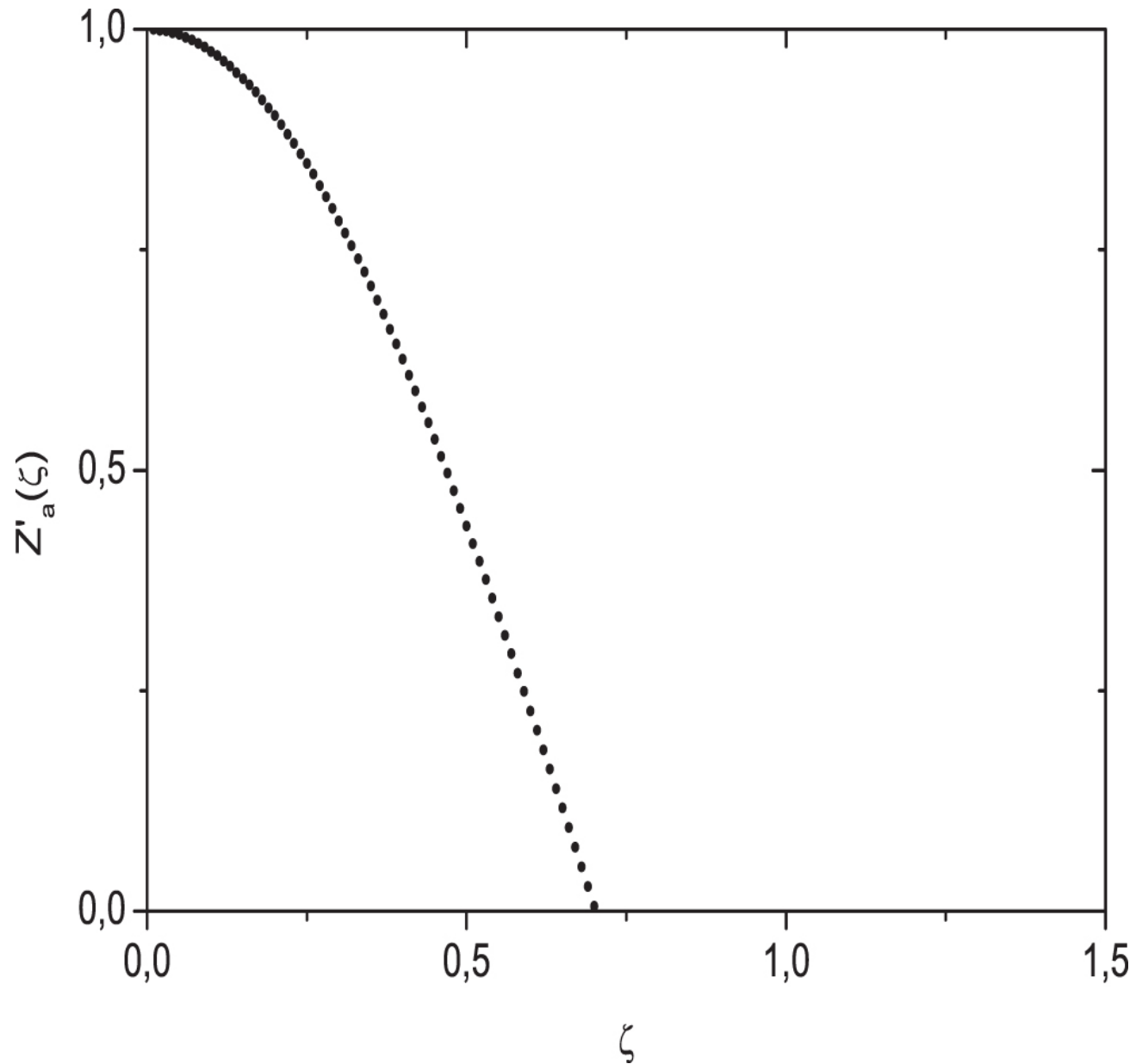
Figure 8. from THE PULSATING PULSAR MAGNETOSPHERE null 2015 APJ 805 106 doi:10.1088/0004-637X/805/2/106 https://dx.doi.org/10.1088/0004-637X/805/2/106 © 2015. The American Astronomical Society. All rights reserved.
