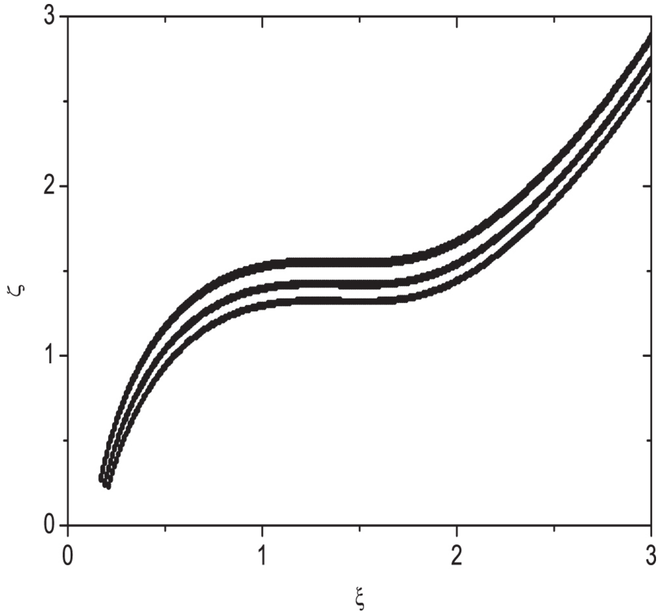
Figure 6. from THE PULSATING PULSAR MAGNETOSPHERE null 2015 APJ 805 106 doi:10.1088/0004-637X/805/2/106 https://dx.doi.org/10.1088/0004-637X/805/2/106 © 2015. The American Astronomical Society. All rights reserved.
