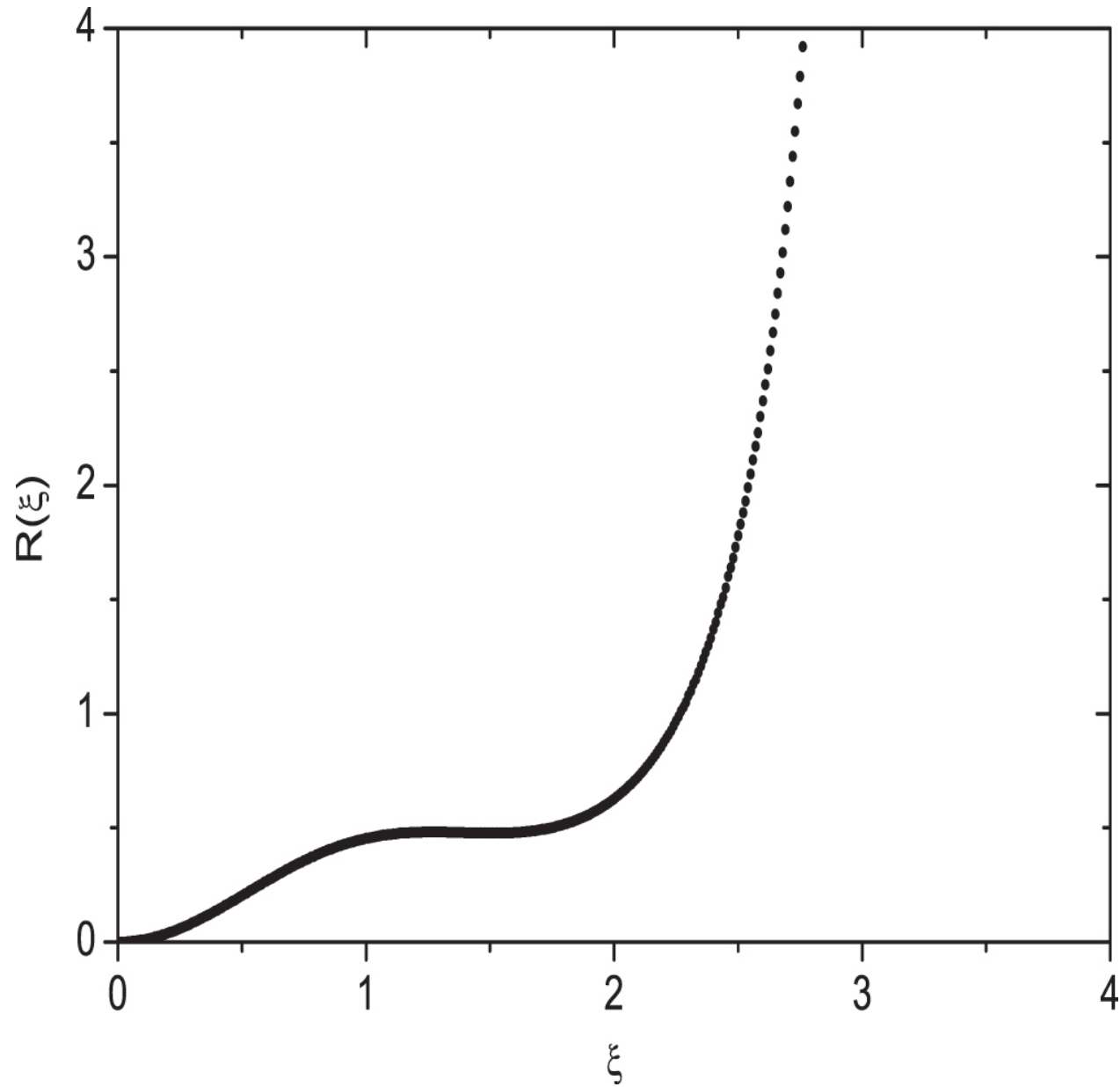
Figure 4. from THE PULSATING PULSAR MAGNETOSPHERE null 2015 APJ 805 106 doi:10.1088/0004-637X/805/2/106 https://dx.doi.org/10.1088/0004-637X/805/2/106 © 2015. The American Astronomical Society. All rights reserved.
