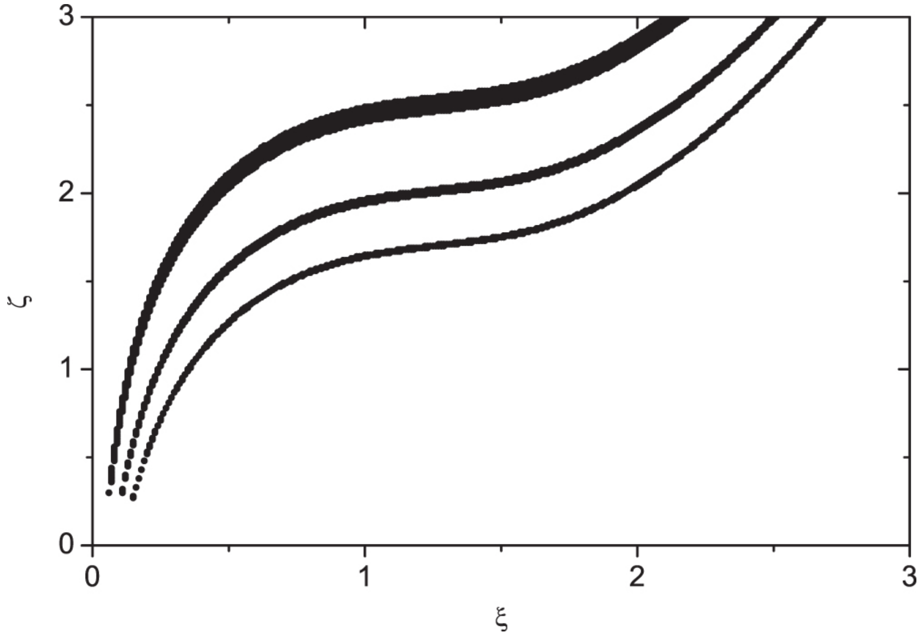
Figure 3. from THE PULSATING PULSAR MAGNETOSPHERE null 2015 APJ 805 106 doi:10.1088/0004-637X/805/2/106 https://dx.doi.org/10.1088/0004-637X/805/2/106 © 2015. The American Astronomical Society. All rights reserved.
