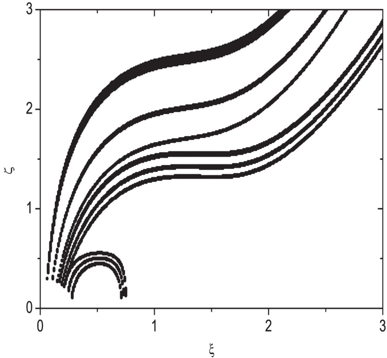
Figure 10. from THE PULSATING PULSAR MAGNETOSPHERE null 2015 APJ 805 106 doi:10.1088/0004-637X/805/2/106 https://dx.doi.org/10.1088/0004-637X/805/2/106 © 2015. The American Astronomical Society. All rights reserved.
