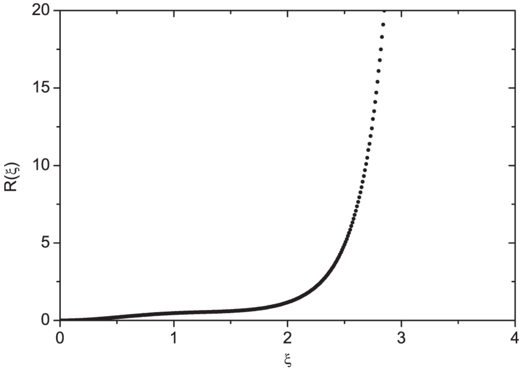
Figure 1. from THE PULSATING PULSAR MAGNETOSPHERE null 2015 APJ 805 106 doi:10.1088/0004-637X/805/2/106 https://dx.doi.org/10.1088/0004-637X/805/2/106 © 2015. The American Astronomical Society. All rights reserved.
