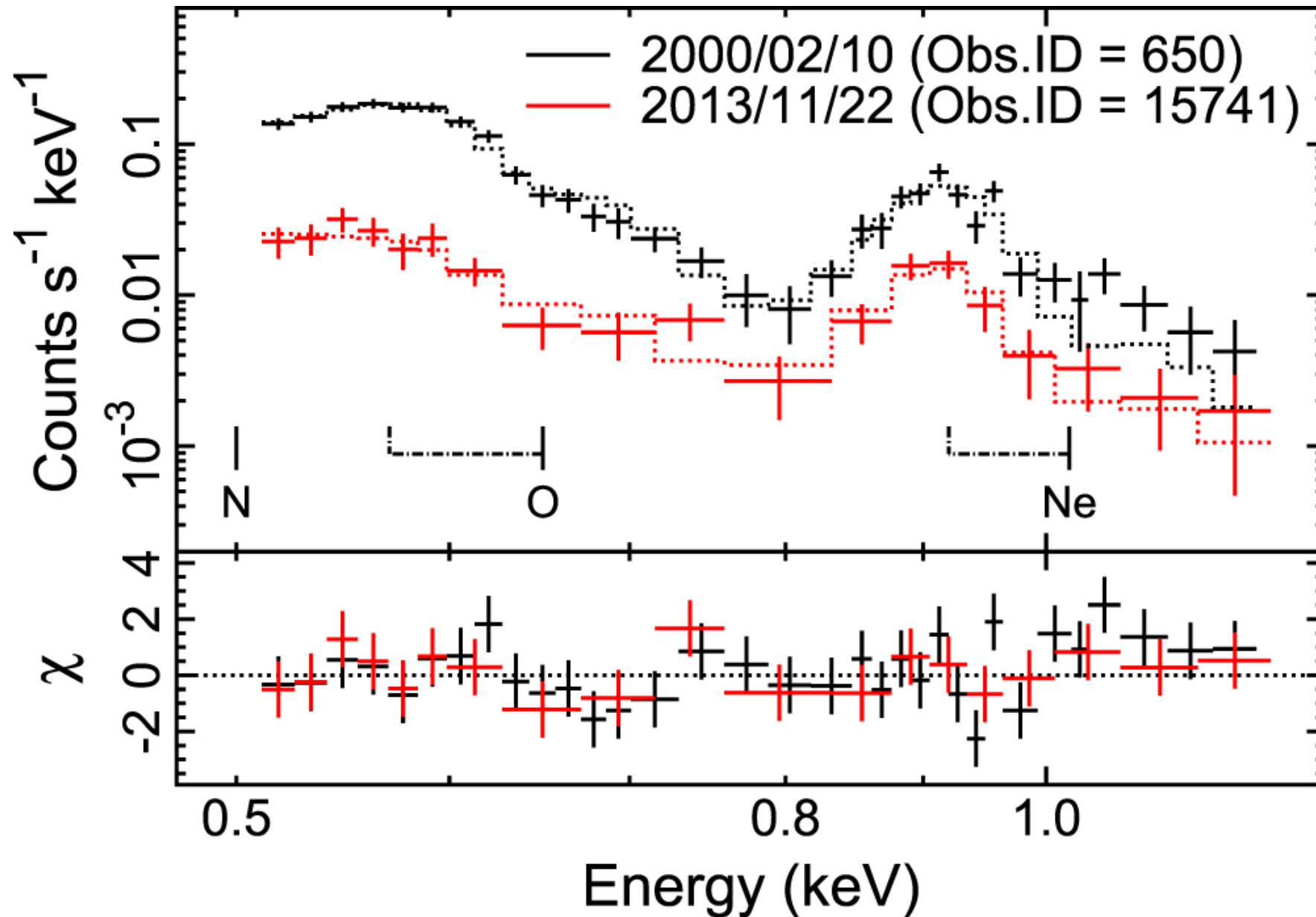
Figure 6. from X-RAY FADING AND EXPANSION IN THE “MINIATURE SUPERNOVA REMNANT” OF GK PERSEI null 2015 APJ 801 92 doi:10.1088/0004-637X/801/2/92 https://dx.doi.org/10.1088/0004-637X/801/2/92 © 2015. The American Astronomical Society. All rights reserved.
