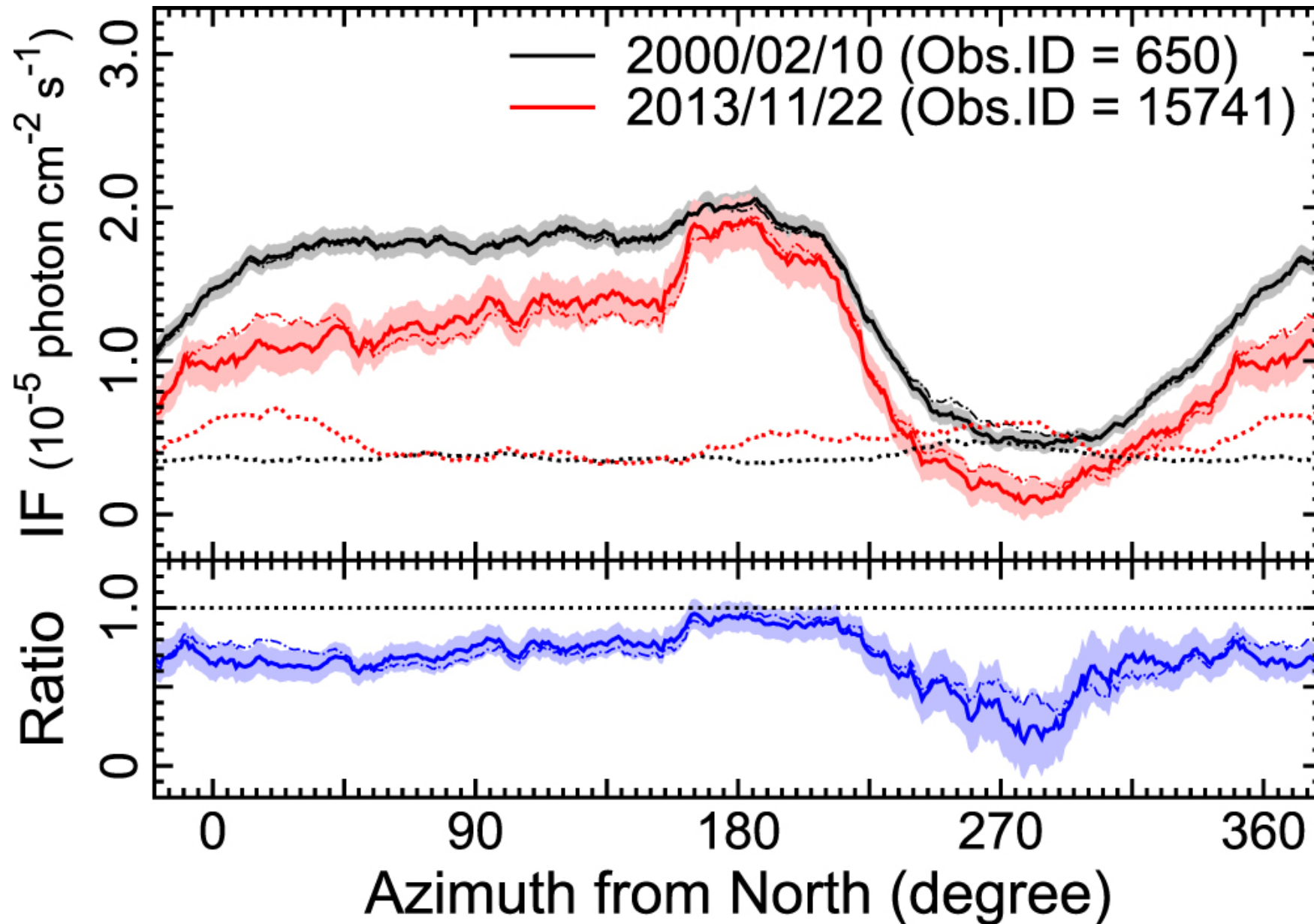
Figure 5. from X-RAY FADING AND EXPANSION IN THE “MINIATURE SUPERNOVA REMNANT” OF GK PERSEI null 2015 APJ 801 92 doi:10.1088/0004-637X/801/2/92 https://dx.doi.org/10.1088/0004-637X/801/2/92 © 2015. The American Astronomical Society. All rights reserved.
