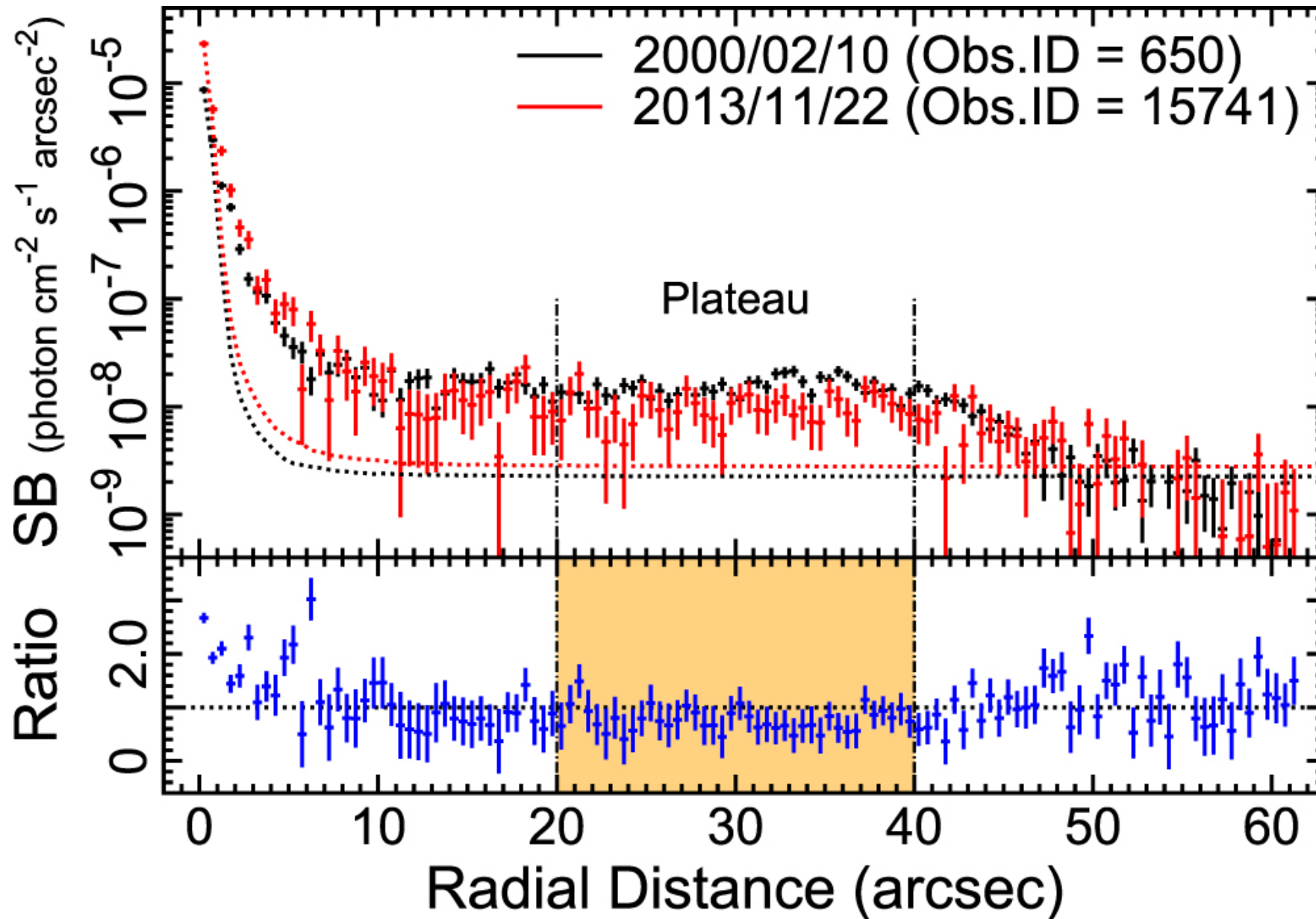
Figure 4. from X-RAY FADING AND EXPANSION IN THE “MINIATURE SUPERNOVA REMNANT” OF GK PERSEI null 2015 APJ 801 92 doi:10.1088/0004-637X/801/2/92 https://dx.doi.org/10.1088/0004-637X/801/2/92 © 2015. The American Astronomical Society. All rights reserved.
