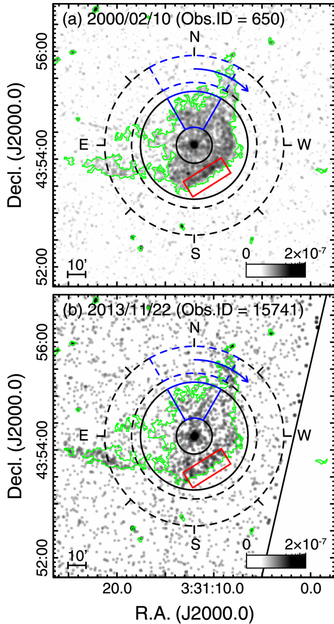
Figure 1. from X-RAY FADING AND EXPANSION IN THE “MINIATURE SUPERNOVA REMNANT” OF GK PERSEI null 2015 APJ 801 92 doi:10.1088/0004-637X/801/2/92 https://dx.doi.org/10.1088/0004-637X/801/2/92 © 2015. The American Astronomical Society. All rights reserved.
