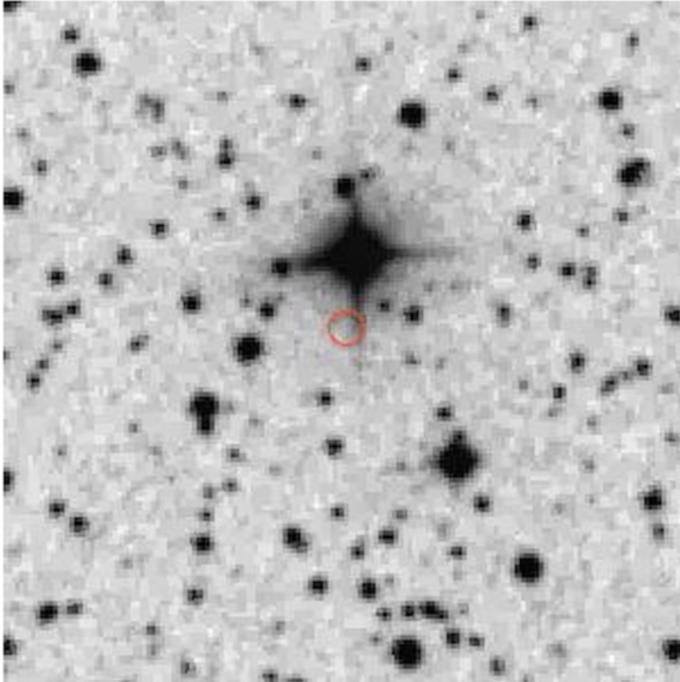
Figure 9. from An Ancient Extrasolar System with Five Sub-Earth-size Planets Campante et al. 2015 ApJ 799 170 doi:10.1088/0004-637X/799/2/170 https://dx.doi.org/10.1088/0004-637X/799/2/170 © 2015. The American Astronomical Society. All rights reserved.
