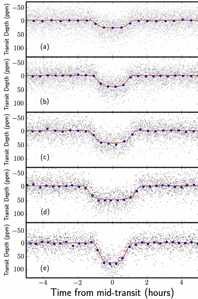
Figure 8. from An Ancient Extrasolar System with Five Sub-Earth-size Planets Campante et al. 2015 ApJ 799 170 doi:10.1088/0004-637X/799/2/170 https://dx.doi.org/10.1088/0004-637X/799/2/170 © 2015. The American Astronomical Society. All rights reserved.
