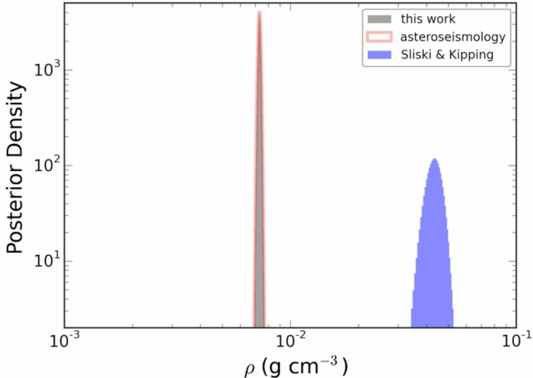
Figure 9. from Radial Velocity Observations and Light Curve Noise Modeling Confirm that Kepler-91b is a Giant Planet Orbiting a Giant Star Barclay et al. 2015 ApJ 800 46 doi:10.1088/0004-637X/800/1/46 https://dx.doi.org/10.1088/0004-637X/800/1/46 © 2015. The American Astronomical Society. All rights reserved.
