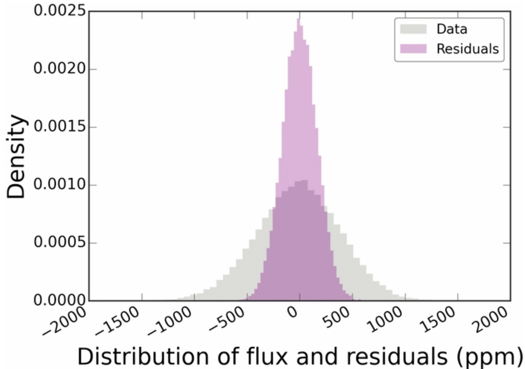
Figure 8. from Radial Velocity Observations and Light Curve Noise Modeling Confirm that Kepler-91b is a Giant Planet Orbiting a Giant Star Barclay et al. 2015 ApJ 800 46 doi:10.1088/0004-637X/800/1/46 https://dx.doi.org/10.1088/0004-637X/800/1/46 © 2015. The American Astronomical Society. All rights reserved.
