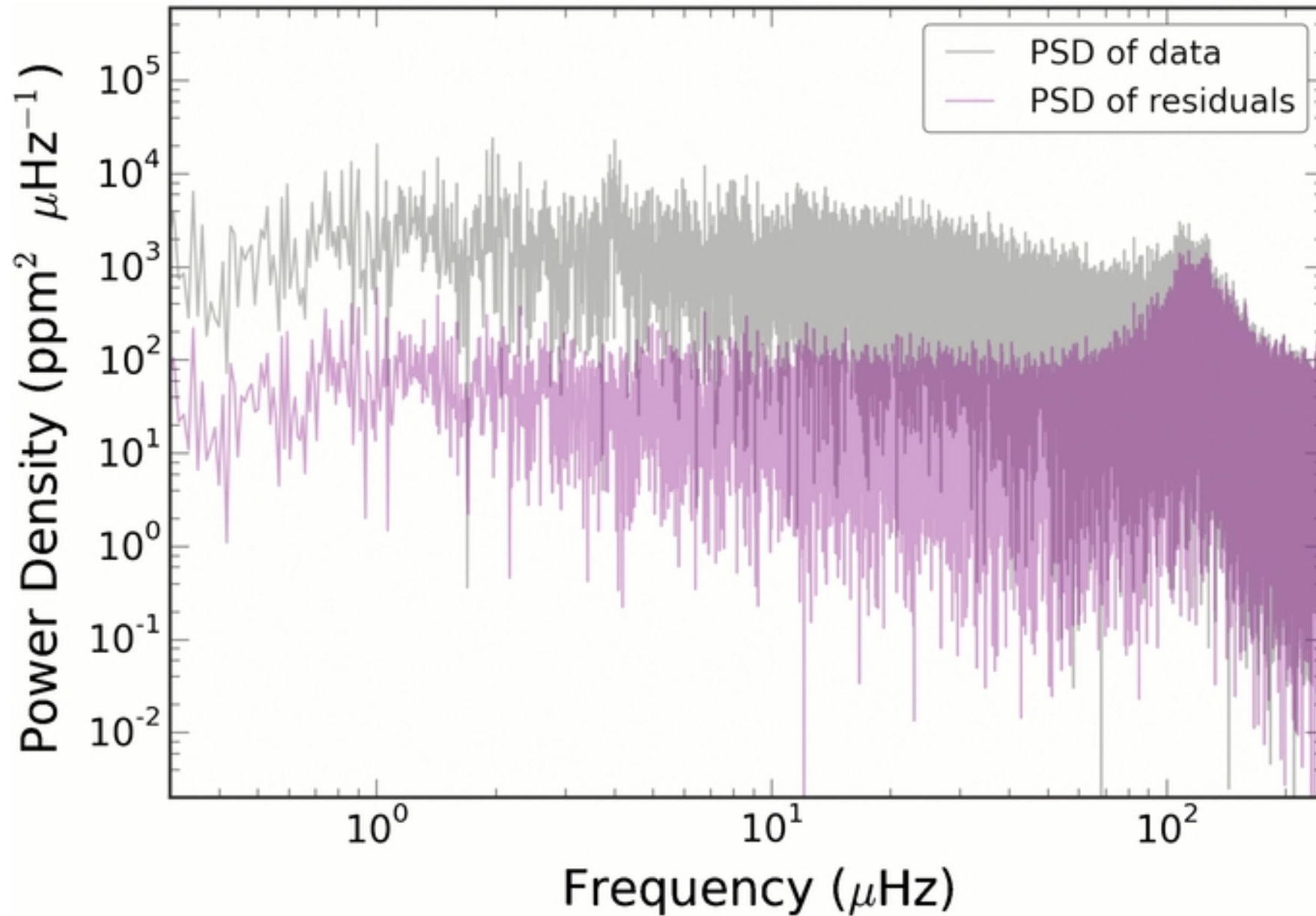
Figure 7. from Radial Velocity Observations and Light Curve Noise Modeling Confirm that Kepler-91b is a Giant Planet Orbiting a Giant Star Barclay et al. 2015 ApJ 800 46 doi:10.1088/0004-637X/800/1/46 https://dx.doi.org/10.1088/0004-637X/800/1/46 © 2015. The American Astronomical Society. All rights reserved.
