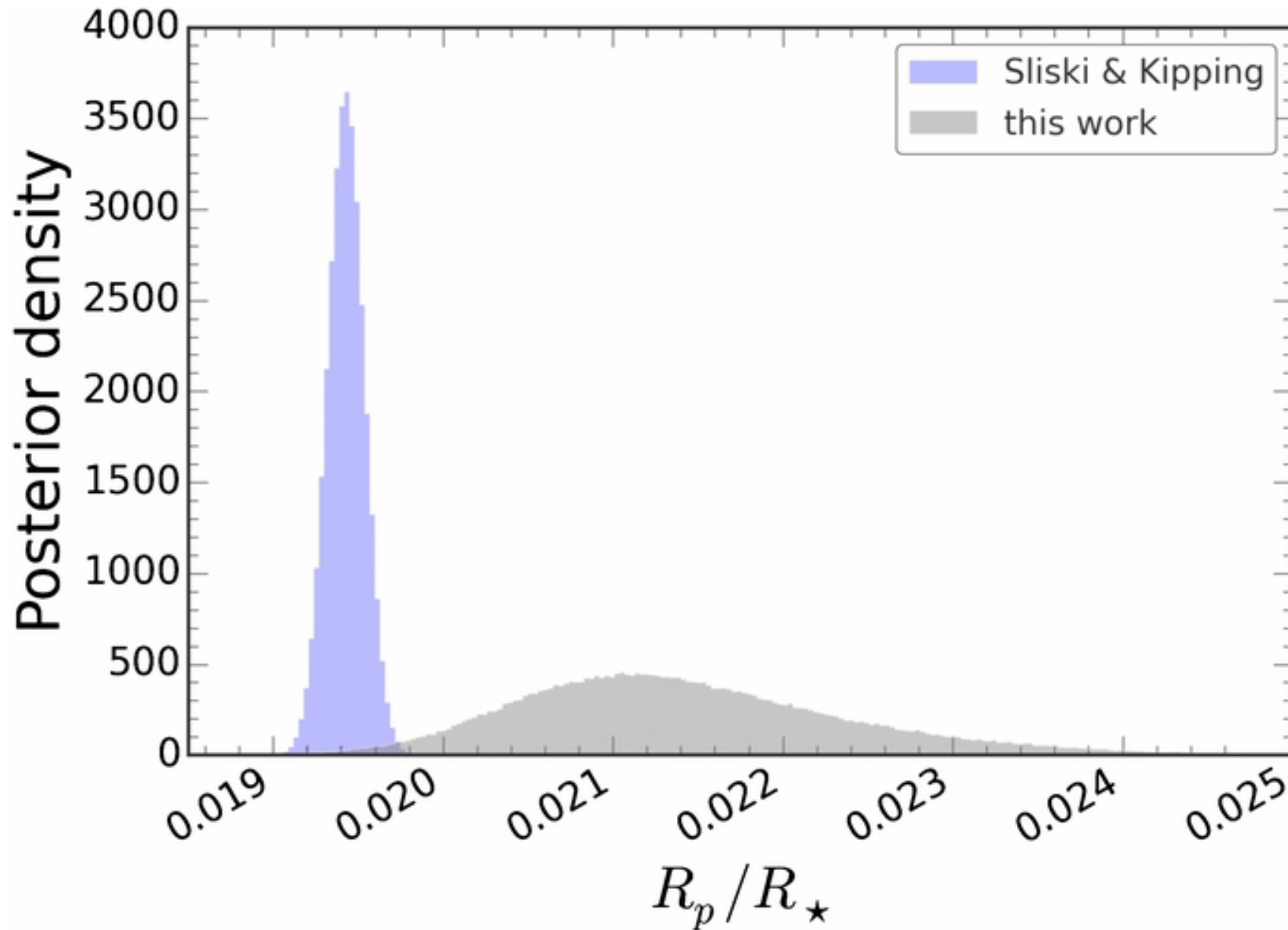
Figure 5. from Radial Velocity Observations and Light Curve Noise Modeling Confirm that Kepler-91b is a Giant Planet Orbiting a Giant Star Barclay et al. 2015 ApJ 800 46 doi:10.1088/0004-637X/800/1/46 https://dx.doi.org/10.1088/0004-637X/800/1/46 © 2015. The American Astronomical Society. All rights reserved.
