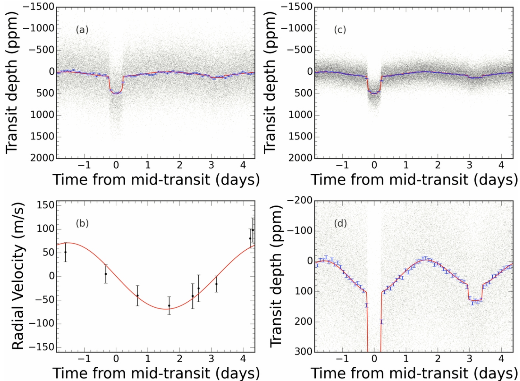
Figure 4. from Radial Velocity Observations and Light Curve Noise Modeling Confirm that Kepler-91b is a Giant Planet Orbiting a Giant Star Barclay et al. 2015 ApJ 800 46 doi:10.1088/0004-637X/800/1/46 https://dx.doi.org/10.1088/0004-637X/800/1/46
