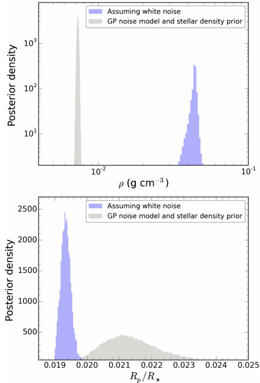
Figure 10. from Radial Velocity Observations and Light Curve Noise Modeling Confirm that Kepler-91b is a Giant Planet Orbiting a Giant Star Barclay et al. 2015 ApJ 800 46 doi:10.1088/0004-637X/800/1/46 https://dx.doi.org/10.1088/0004-637X/800/1/46 © 2015. The American Astronomical Society. All rights reserved.
