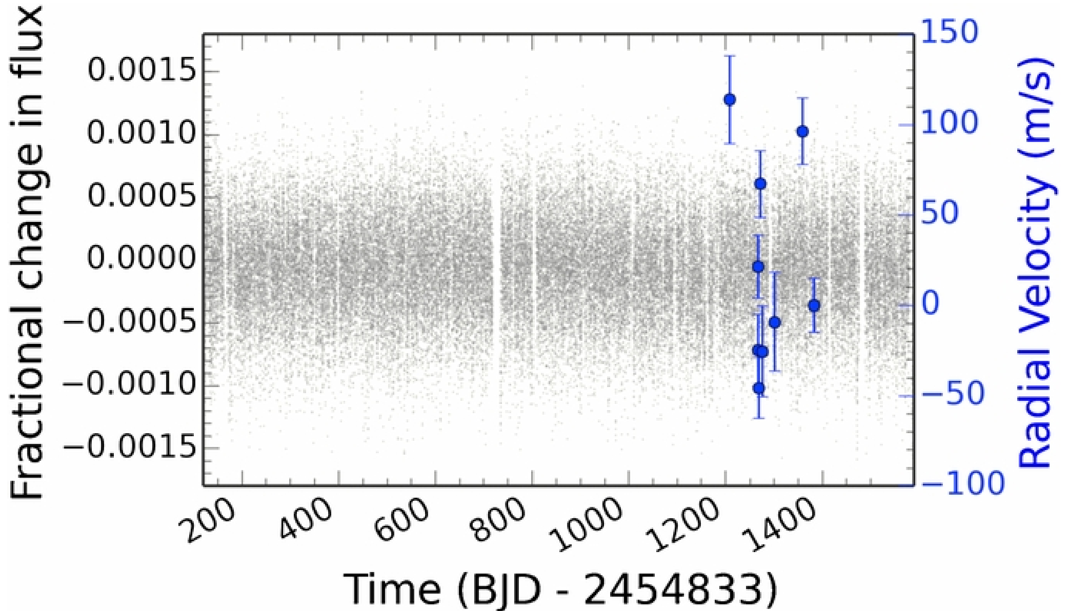
Figure 1. from Radial Velocity Observations and Light Curve Noise Modeling Confirm that Kepler-91b is a Giant Planet Orbiting a Giant Star Barclay et al. 2015 ApJ 800 46 doi:10.1088/0004-637X/800/1/46 https://dx.doi.org/10.1088/0004-637X/800/1/46 © 2015. The American Astronomical Society. All rights reserved.
