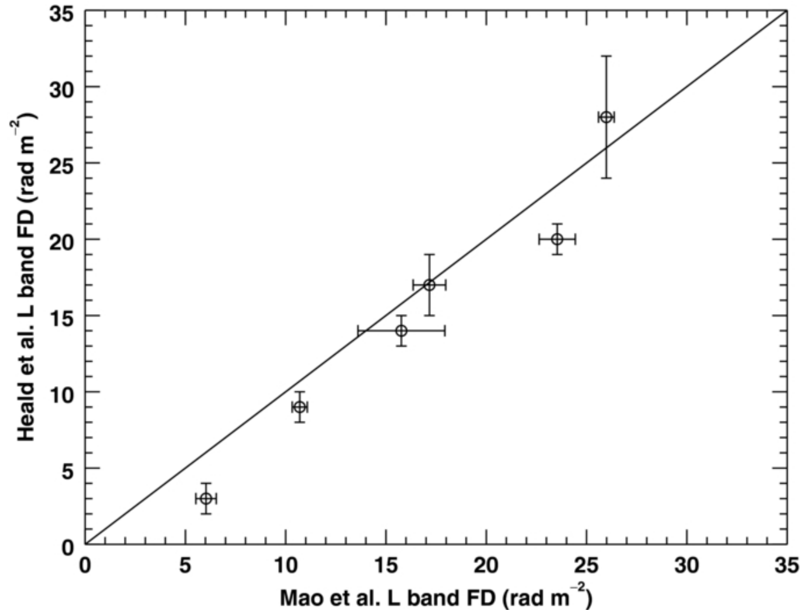
Figure 6. from Properties of the Magneto-ionic Medium in the Halo of M51 Revealed by Wide-band Polarimetry Mao et al. 2015 ApJ 800 92 doi:10.1088/0004-637X/800/2/92 https://dx.doi.org/10.1088/0004-637X/800/2/92 © 2015. The American Astronomical Society. All rights reserved.
