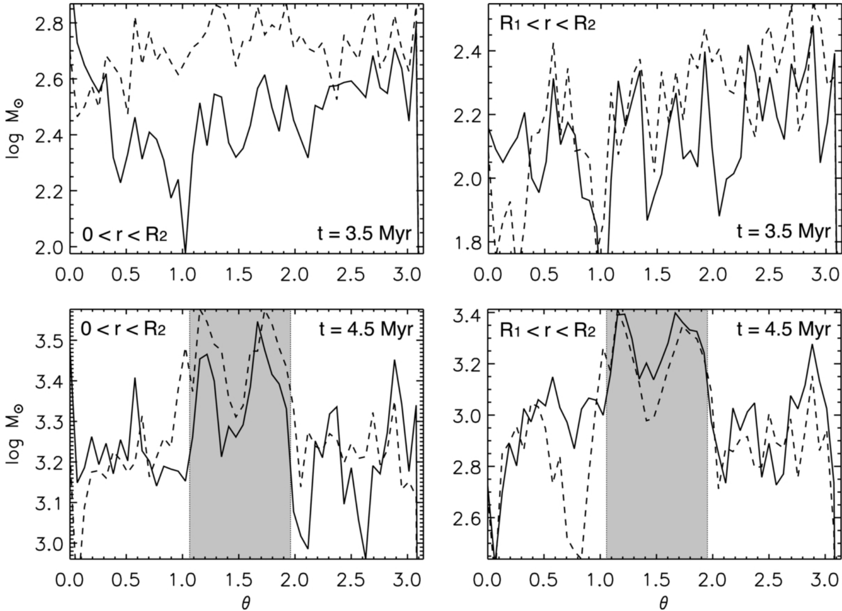
Figure 8. from A Young Giant Molecular Cloud Formed at the Interface of Two Colliding Supershells: Observations Meet Simulations Dawson et al. 2015 ApJ 799 64 doi:10.1088/0004-637X/799/1/64 https://dx.doi.org/10.1088/0004-637X/799/1/64 © 2015. The American Astronomical Society. All rights reserved.
