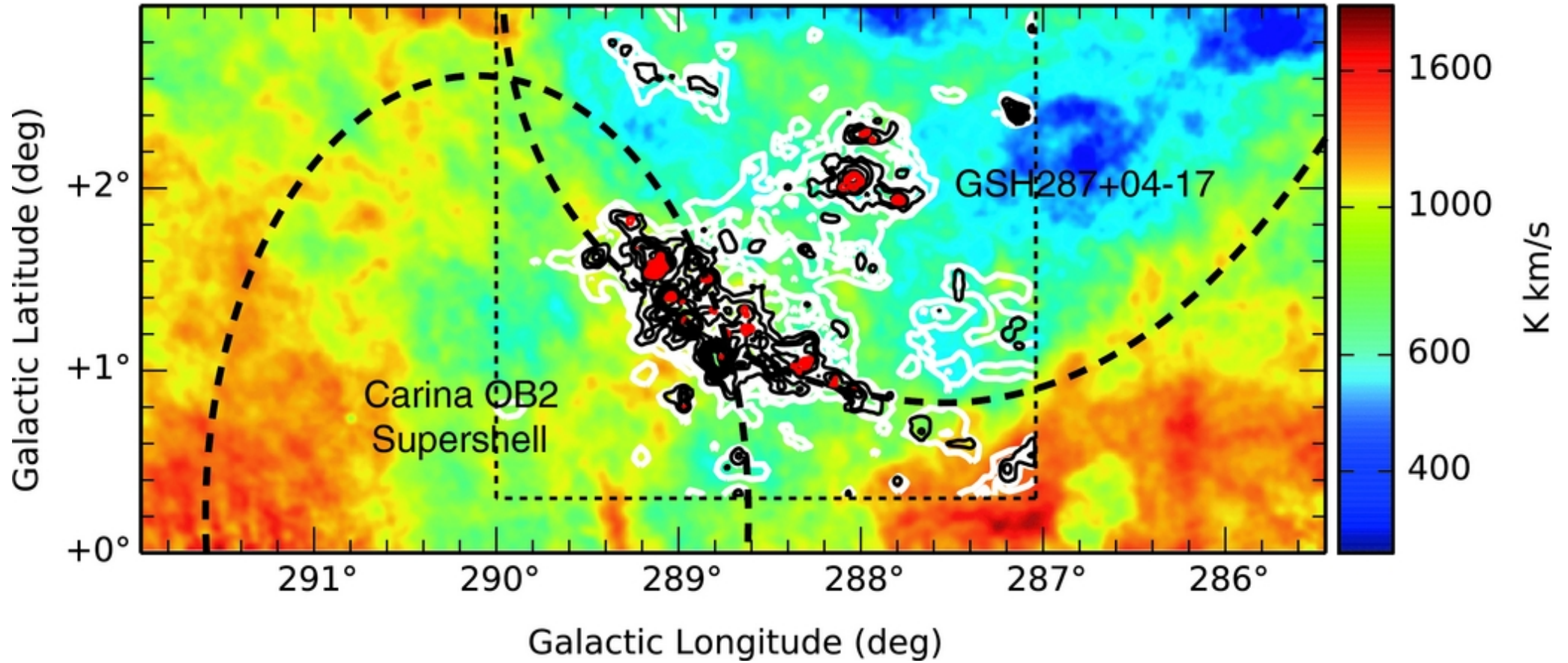
Figure 1. from A Young Giant Molecular Cloud Formed at the Interface of Two Colliding Supershells: Observations Meet Simulations Dawson et al. 2015 ApJ 799 64 doi:10.1088/0004-637X/799/1/64 https://dx.doi.org/10.1088/0004-637X/799/1/64 © 2015. The American Astronomical Society. All rights reserved.
