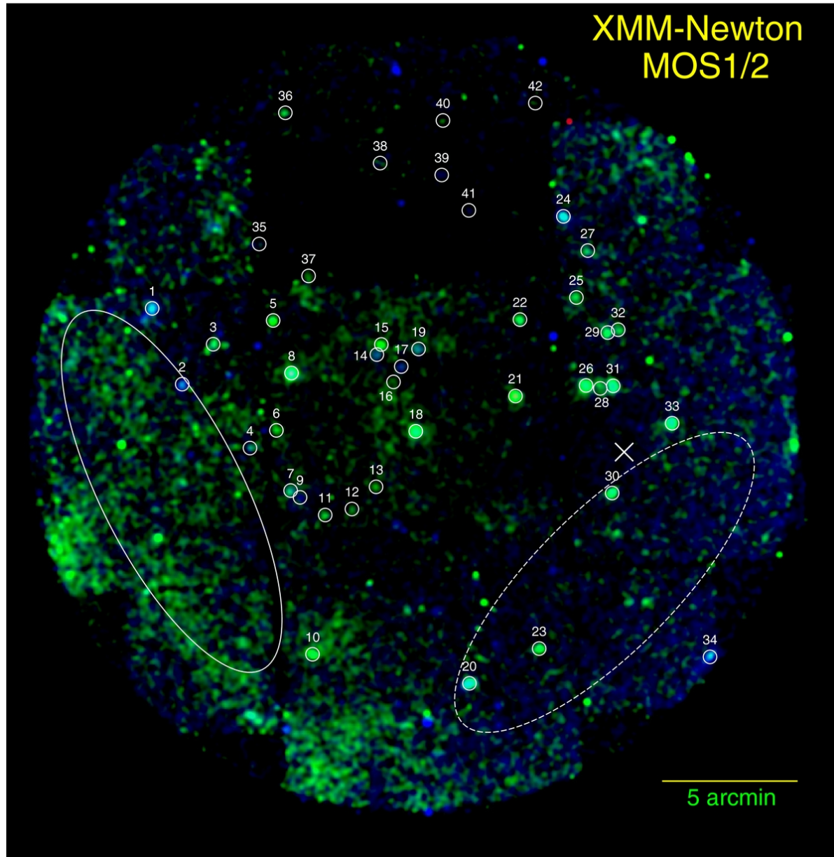
Figure 1. from A Detailed X-Ray Investigation of PSR J2021+4026 and the -Cygni Supernova Remnant Hui et al. 2015 ApJ 799 76 doi:10.1088/0004-637X/799/1/76 https://dx.doi.org/10.1088/0004-637X/799/1/76 © 2015. The American Astronomical Society. All rights reserved.
