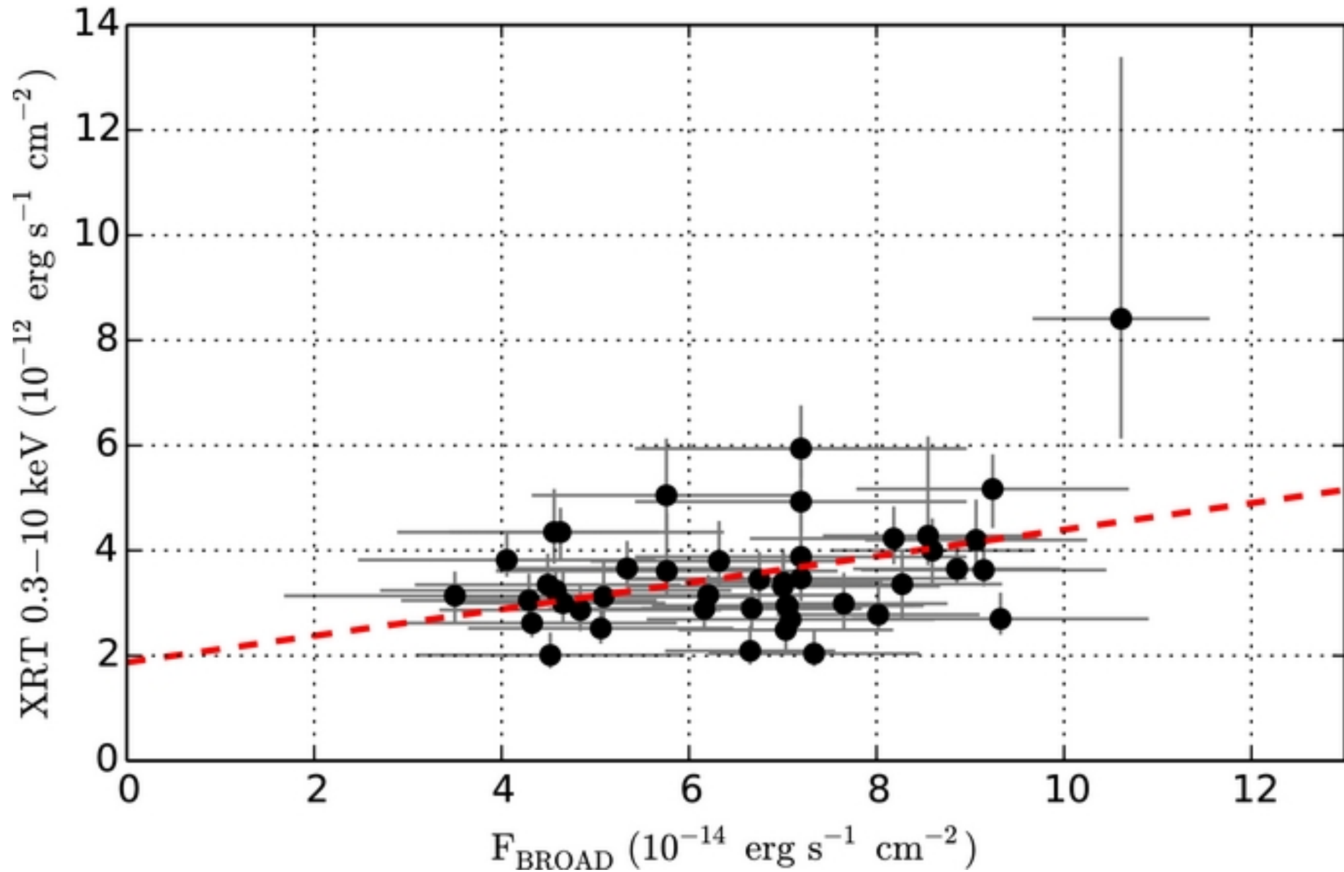
Figure 7. from Short-timescale Monitoring of the X-Ray, UV, and Broad Double-peak Emission Line of the Nucleus of NGC 1097 Schimoia et al. 2015 ApJ 800 63 doi:10.1088/0004-637X/800/1/63 https://dx.doi.org/10.1088/0004-637X/800/1/63 © 2015. The American Astronomical Society. All rights reserved.
