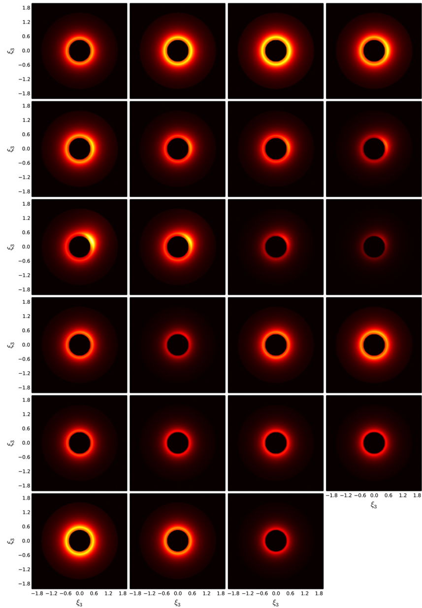
Figure 6. from Short-timescale Monitoring of the X-Ray, UV, and Broad Double-peak Emission Line of the Nucleus of NGC 1097 Schimoia et al. 2015 ApJ 800 63 doi:10.1088/0004-637X/800/1/63 https://dx.doi.org/10.1088/0004-637X/800/1/63
