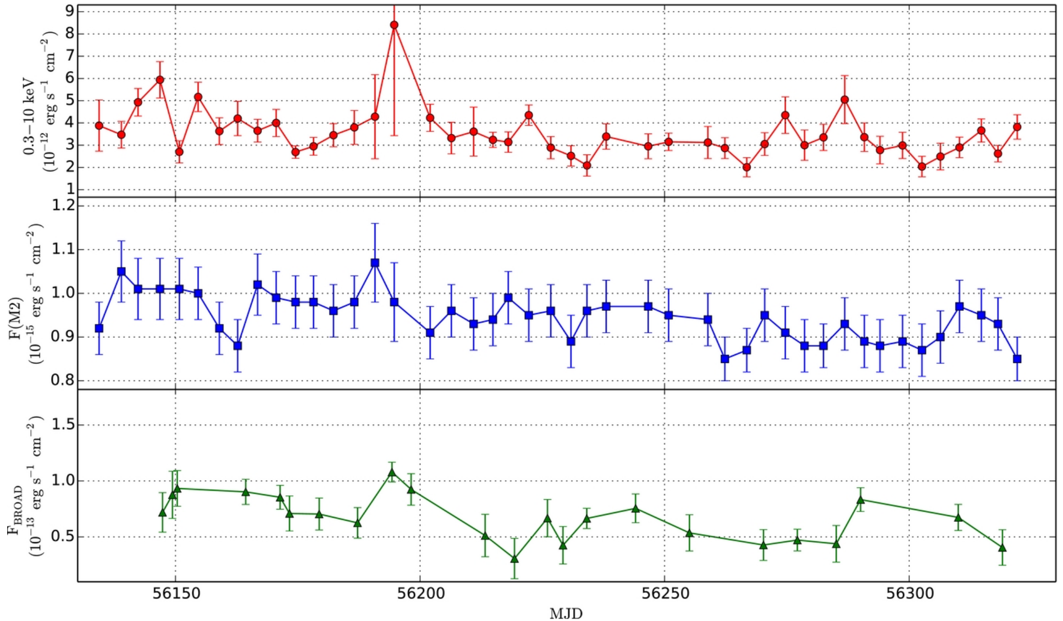
Figure 4. from Short-timescale Monitoring of the X-Ray, UV, and Broad Double-peak Emission Line of the Nucleus of NGC 1097 Schimoia et al. 2015 ApJ 800 63 doi:10.1088/0004-637X/800/1/63 https://dx.doi.org/10.1088/0004-637X/800/1/63 © 2015. The American Astronomical Society. All rights reserved.
