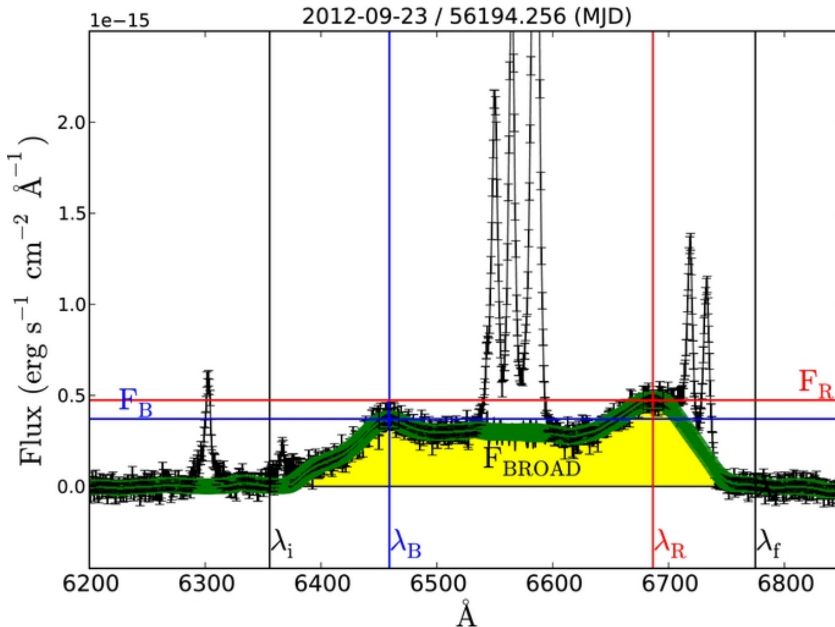
Figure 3. from Short-timescale Monitoring of the X-Ray, UV, and Broad Double-peak Emission Line of the Nucleus of NGC 1097 Schimoia et al. 2015 ApJ 800 63 doi:10.1088/0004-637X/800/1/63 https://dx.doi.org/10.1088/0004-637X/800/1/63 © 2015. The American Astronomical Society. All rights reserved.
