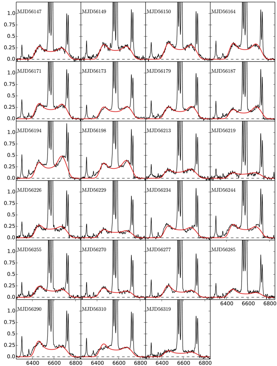
Figure 2. from Short-timescale Monitoring of the X-Ray, UV, and Broad Double-peak Emission Line of the Nucleus of NGC 1097 Schimoia et al. 2015 ApJ 800 63 doi:10.1088/0004-637X/800/1/63 https://dx.doi.org/10.1088/0004-637X/800/1/63
