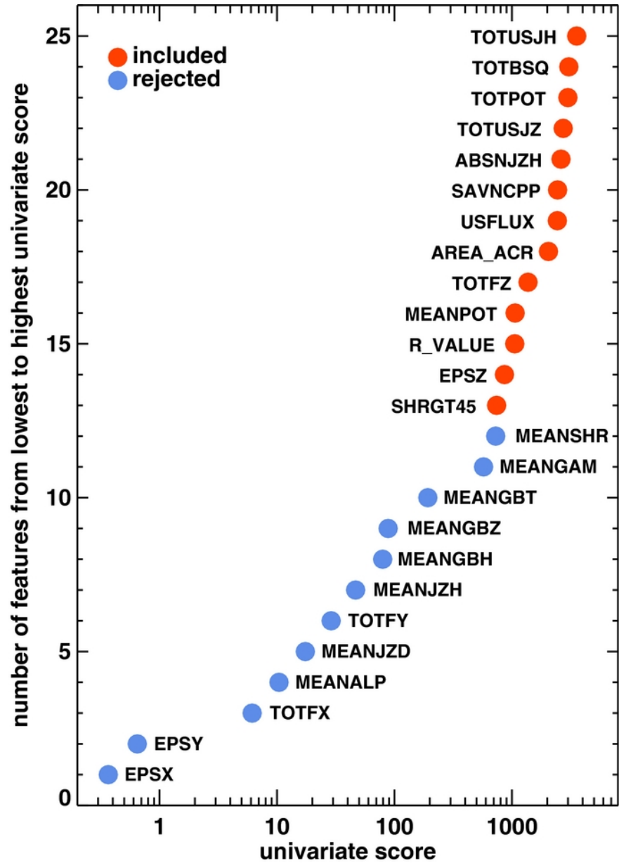
Figure 3. from Solar Flare Prediction Using SDO/HMI Vector Magnetic Field Data with a Machine-learning Algorithm Bobra & Couvidat 2015 ApJ 798 135 doi:10.1088/0004-637X/798/2/135 https://dx.doi.org/10.1088/0004-637X/798/2/135 © 2015. The American Astronomical Society. All rights reserved.
