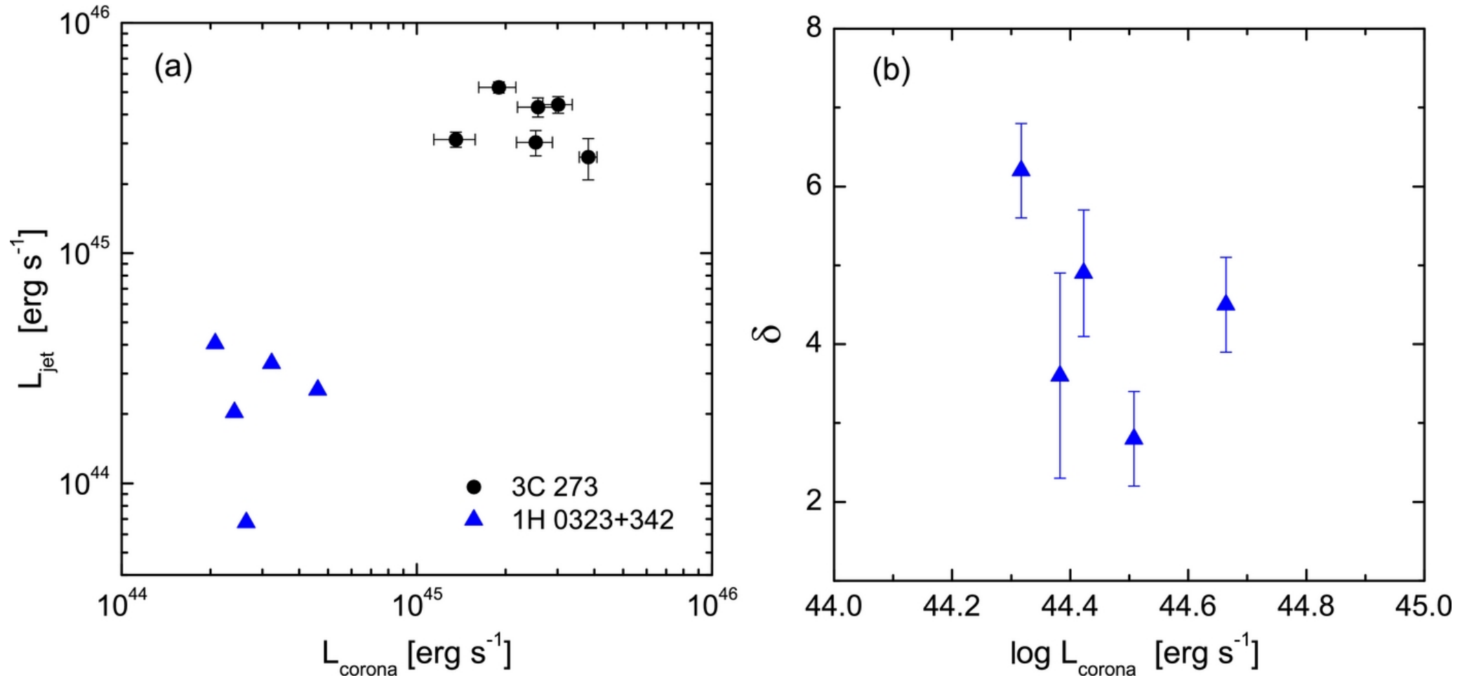
Figure 8. from Jet Properties of GeV-selected Radio-loud Narrow-line Seyfert 1 Galaxies and Possible Connection to Their Disk and Corona Sun et al. 2015 ApJ 798 43 doi:10.1088/0004-637X/798/1/43 https://dx.doi.org/10.1088/0004-637X/798/1/43 © 2015. The American Astronomical Society. All rights reserved.
