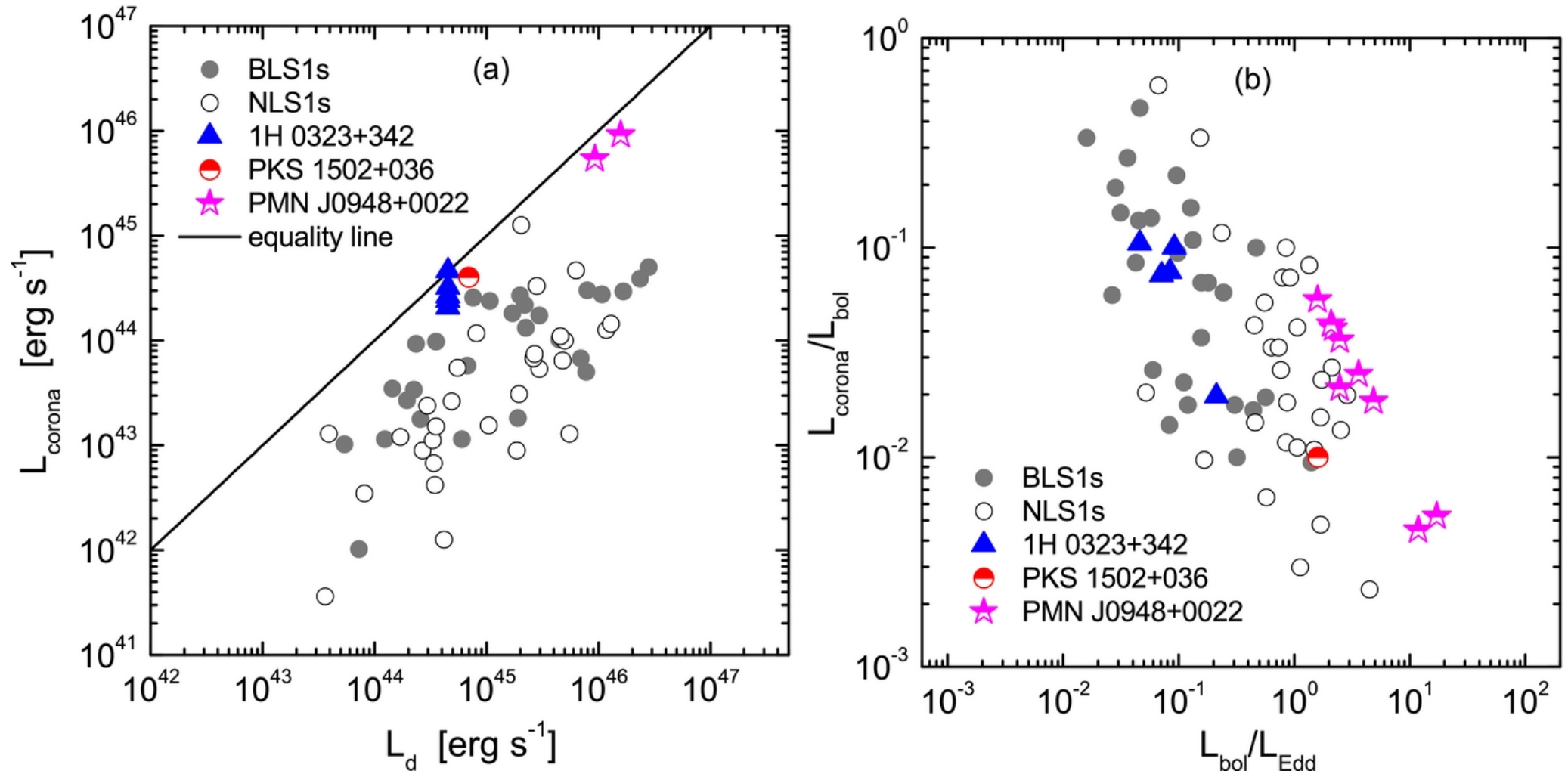
Figure 7. from Jet Properties of GeV-selected Radio-loud Narrow-line Seyfert 1 Galaxies and Possible Connection to Their Disk and Corona Sun et al. 2015 ApJ 798 43 doi:10.1088/0004-637X/798/1/43 https://dx.doi.org/10.1088/0004-637X/798/1/43 © 2015. The American Astronomical Society. All rights reserved.
